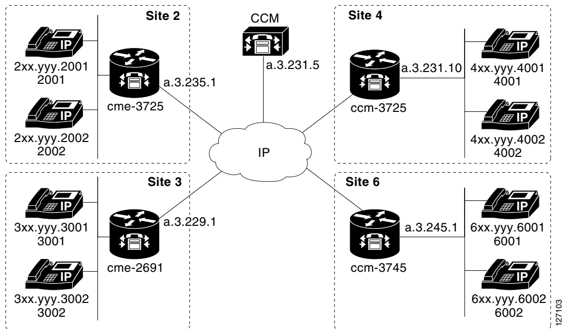
Figure 1 Network Diagram (Direct IP Addressing)
