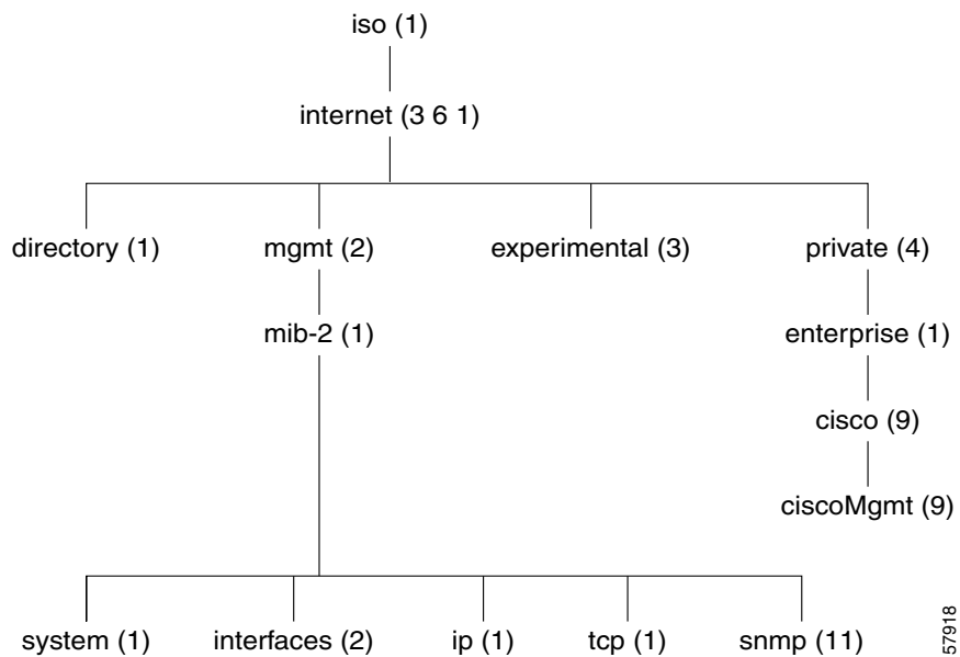
Figure A-1 MIB Tree
