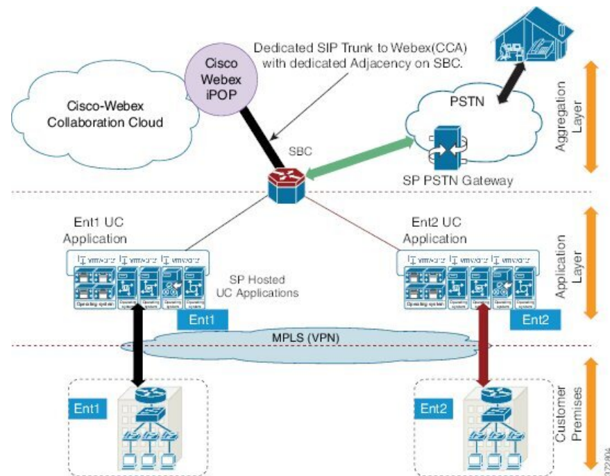
Figure 5: Cisco Webex Collaboration Cloud Audio Architecture
