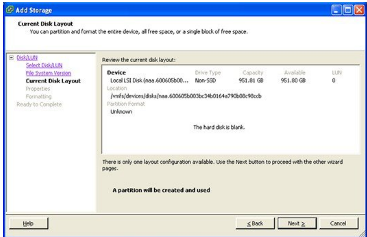
Figure 5: Verify Details
