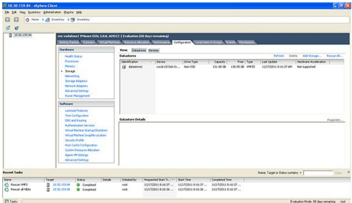
Figure 1: Select Storage
