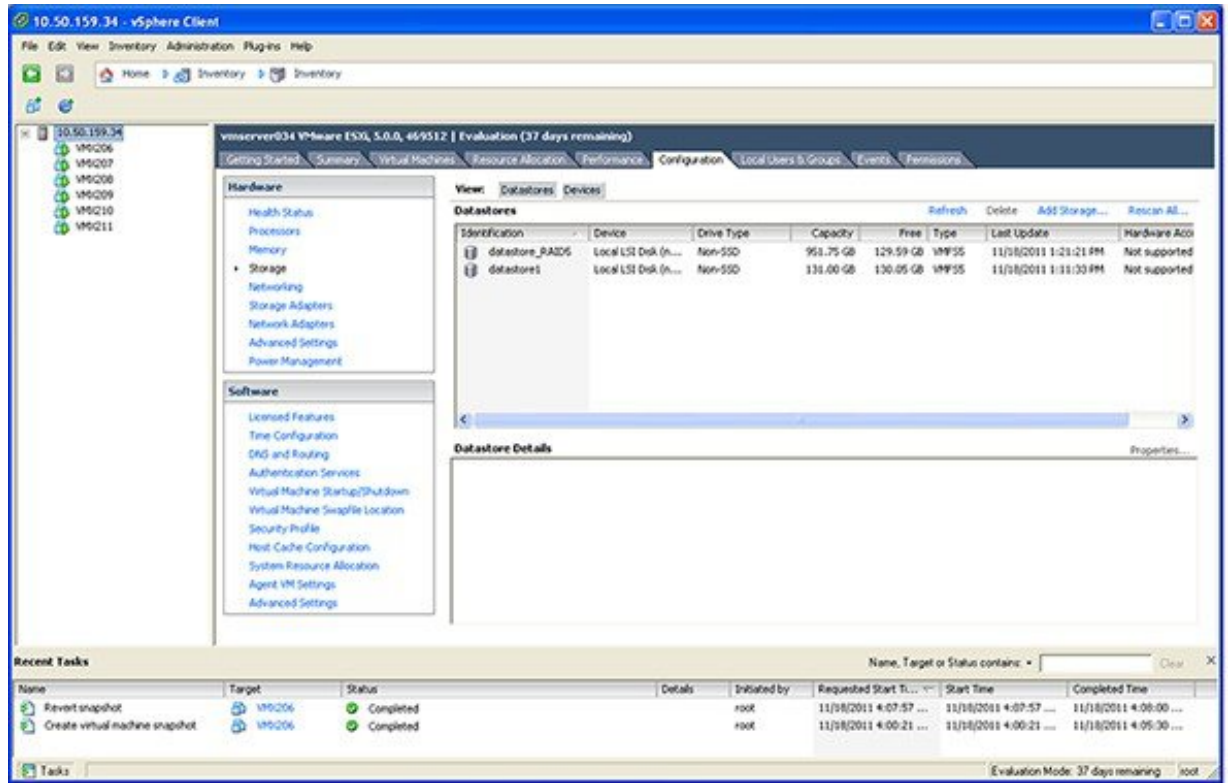
Figure 9: New Datastore
