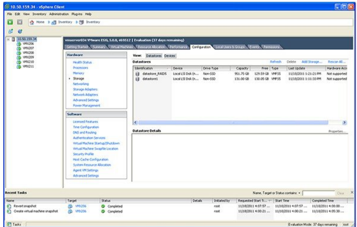
Figure 9: New Datastore
