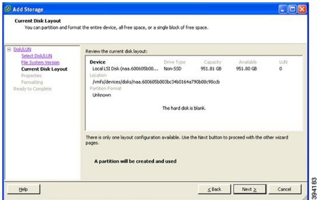
Figure 5: Verify Details
