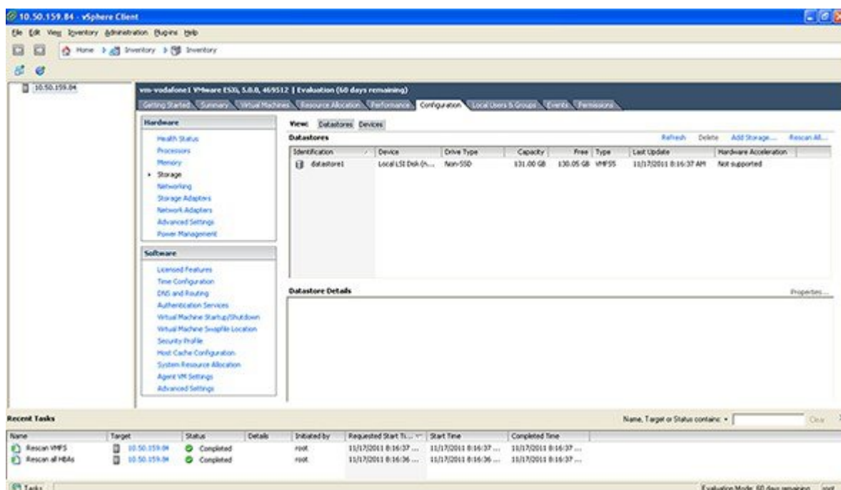
Figure 1: Select Storage
