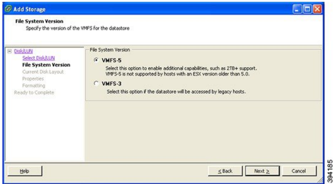
Figure 4: Select VMFS-5
