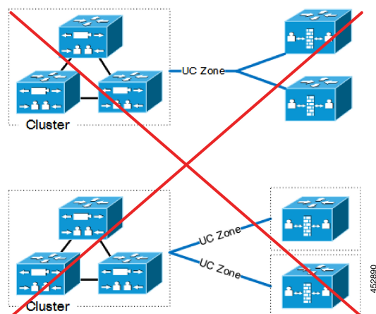
Figure 10: Unclustered or Many-to-One Traversal Connections
