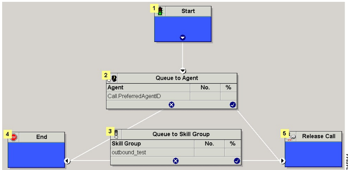
Figure 11: Sample Script for Agent Campaign with Personal Callback
