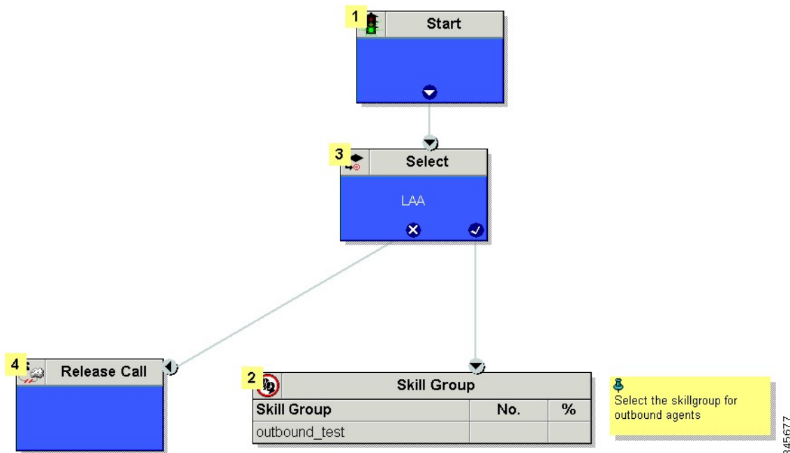
Figure 9: Sample Script for Agent Campaign Without Personal Callback (Using Select Node)
