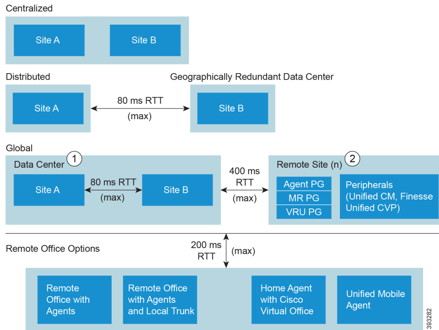
Figure 33: Topologies
