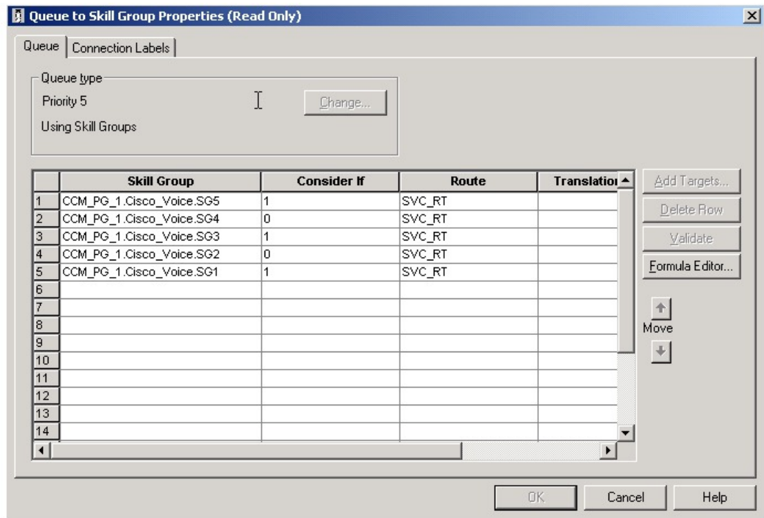
Figure 5: Queue to Skill Group Properties
