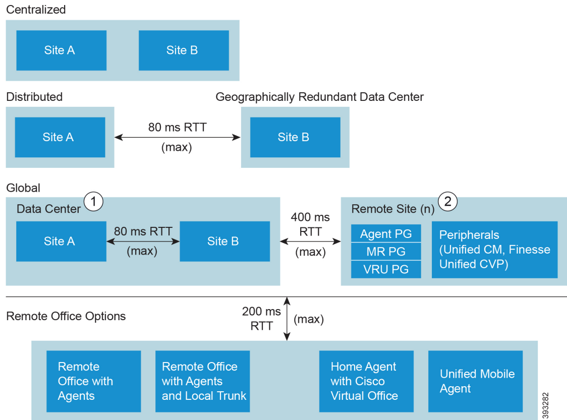
Figure 11: Reference Design Topologies
