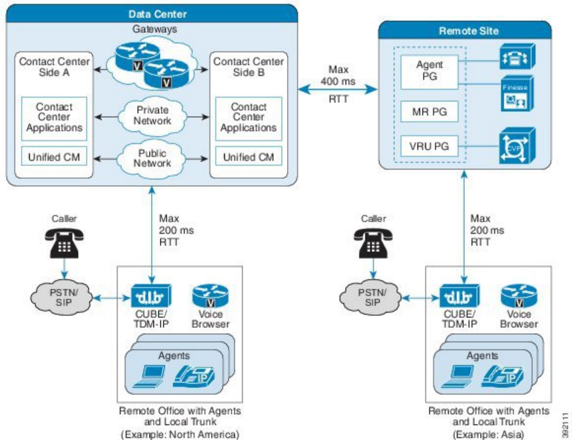
Figure 39: Global Deployment Topology
