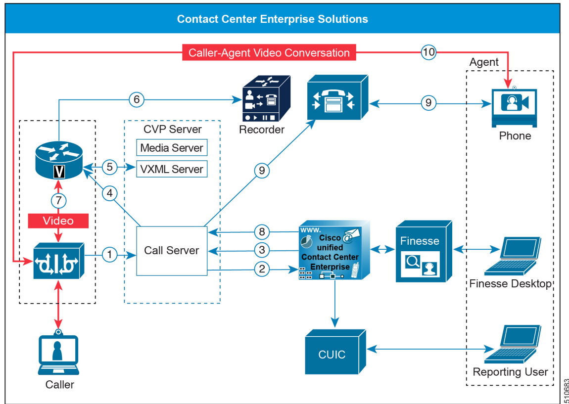
Figure 30: Video Call Flow
