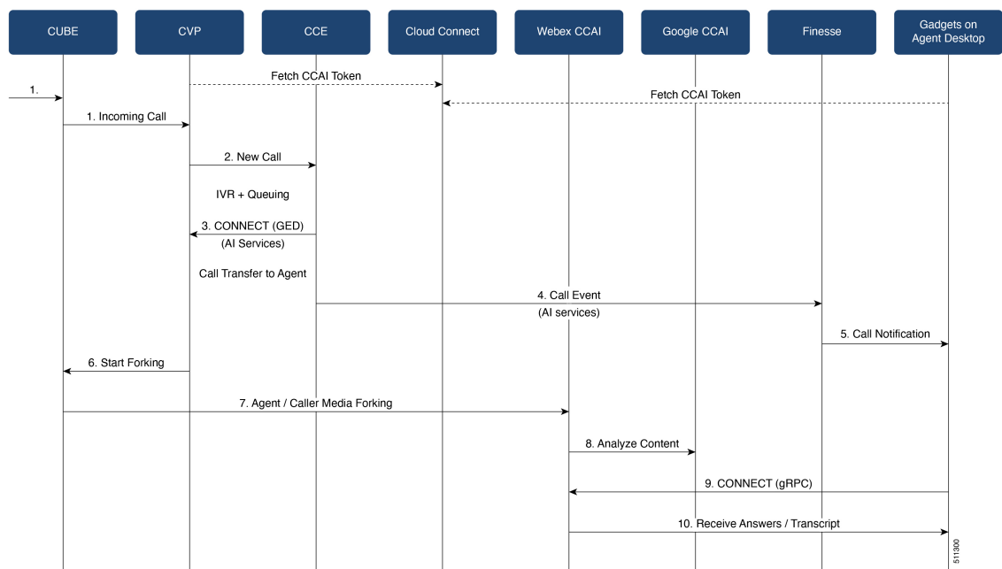
Figure 4: Contact Center AI Services Call Flow Diagram
