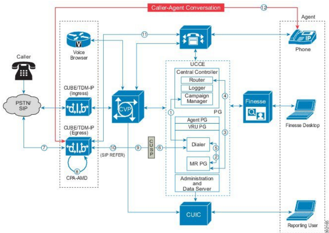
Figure 7: SIP Dialer Agent Campaign Call Flow
