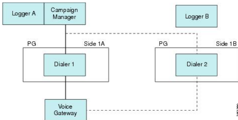
Figure 9: Single Gateway Deployment for SIP Dialer
