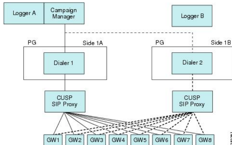
Figure 10: Multiple Gateway Deployment for SIP Dialer
