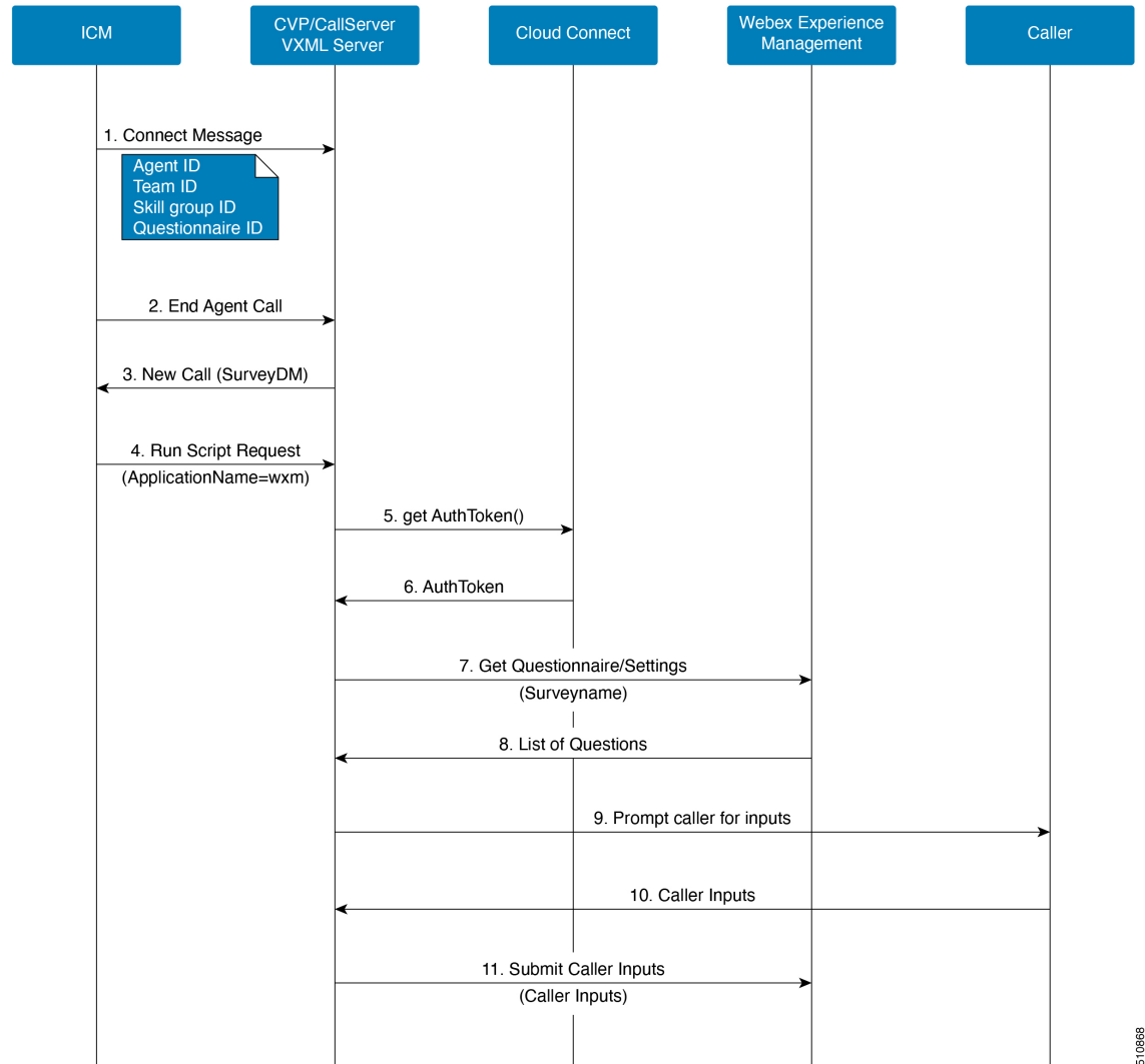
Figure 17: Voice Survey Call Flow
