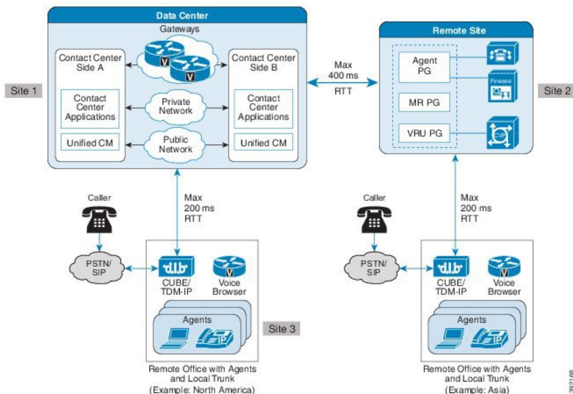
Figure 11: Distributed Deployment Example for Agent-Based Campaign
