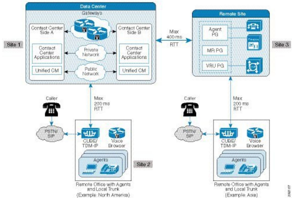
Figure 13: Distributed Outbound SIP Dialer Deployment for Transfer to a VRU Campaign with CVP
