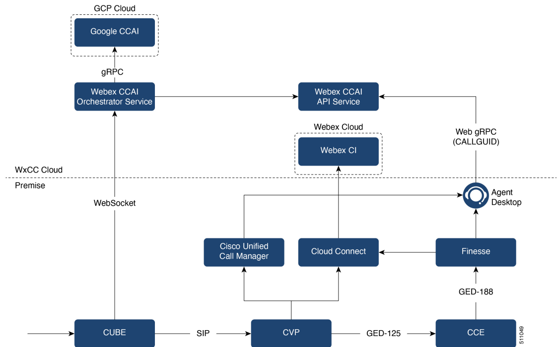
Figure 3: Contact Center AI Services Architecture
