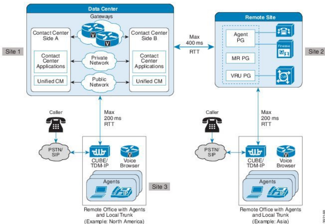
Figure 12: Distributed Outbound SIP Dialer Deployment for an Agent-Based Campaign
