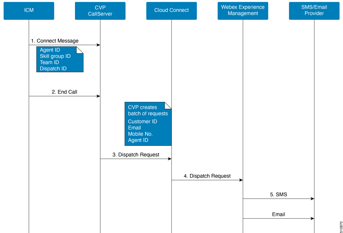
Figure 18: Email/SMS Survey Call Flow
