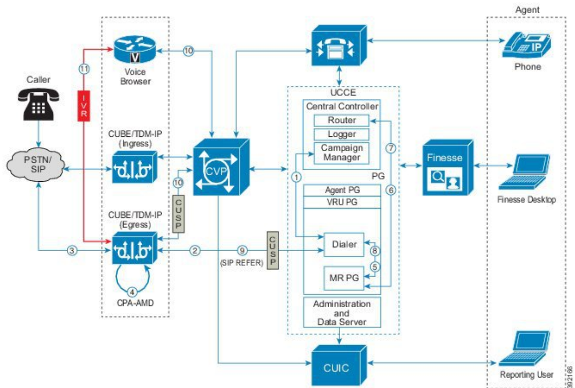
Figure 8: SIP Dialer Unattended VRU Campaign Call Flow
