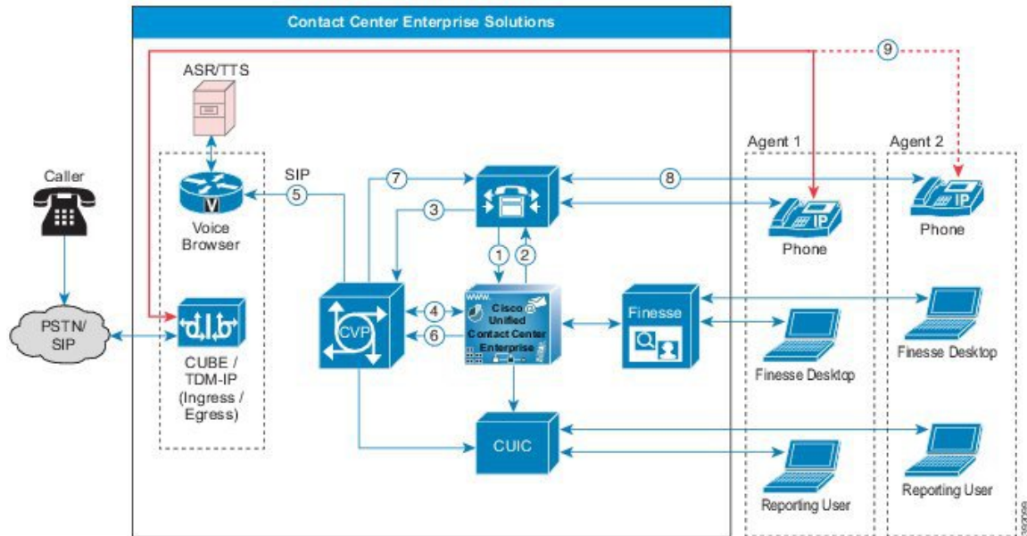
Figure 30: Blind Transfer Call Flow with VRU and Queue to a Second Agent
