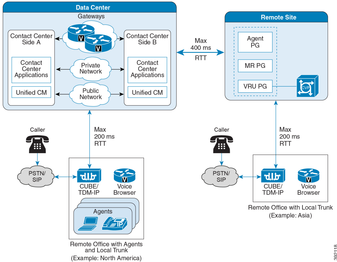
Figure 36: Remote CVP Deployment Topology
