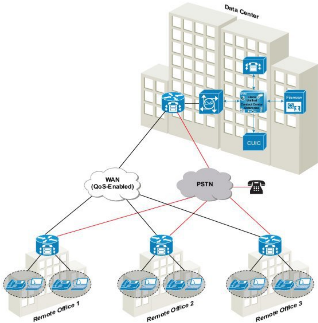
Figure 40: Remote Offices with Agents and Local Trunks
