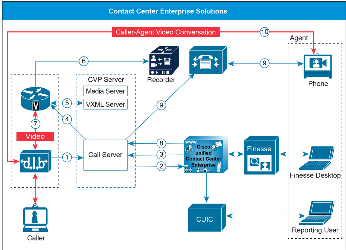
Figure 29: Video Call Flow
