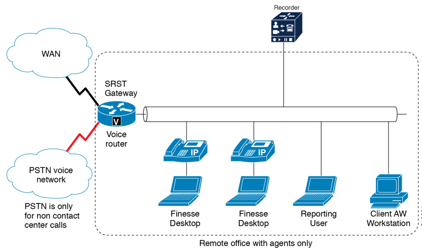
Figure 39: Remote Office with Agents—Physical View
