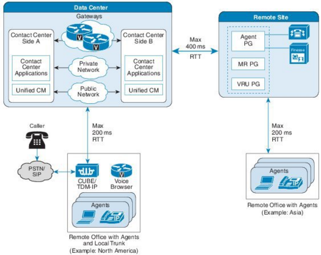
Figure 37: Remote Unified Communications Manager Clusters Topology
