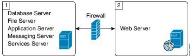
Figure 19: Collocated Deployment
