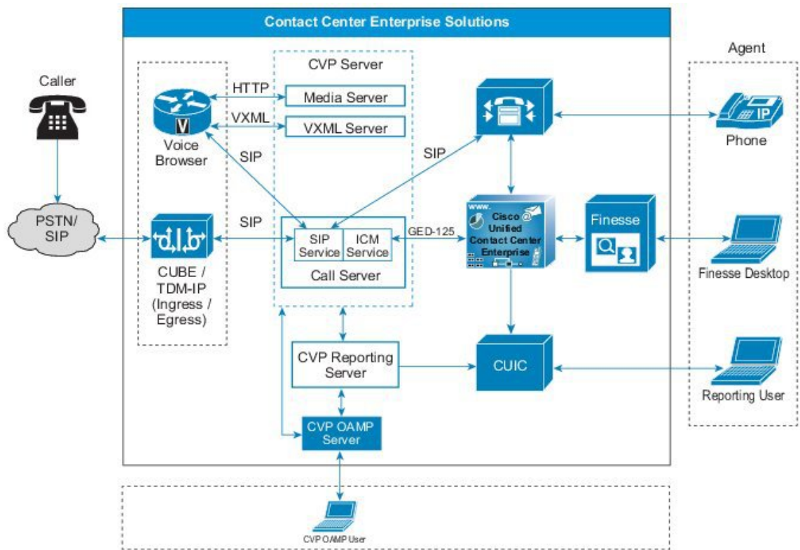
Figure 4: Unified CVP in a Contact Center Enterprise Solution
