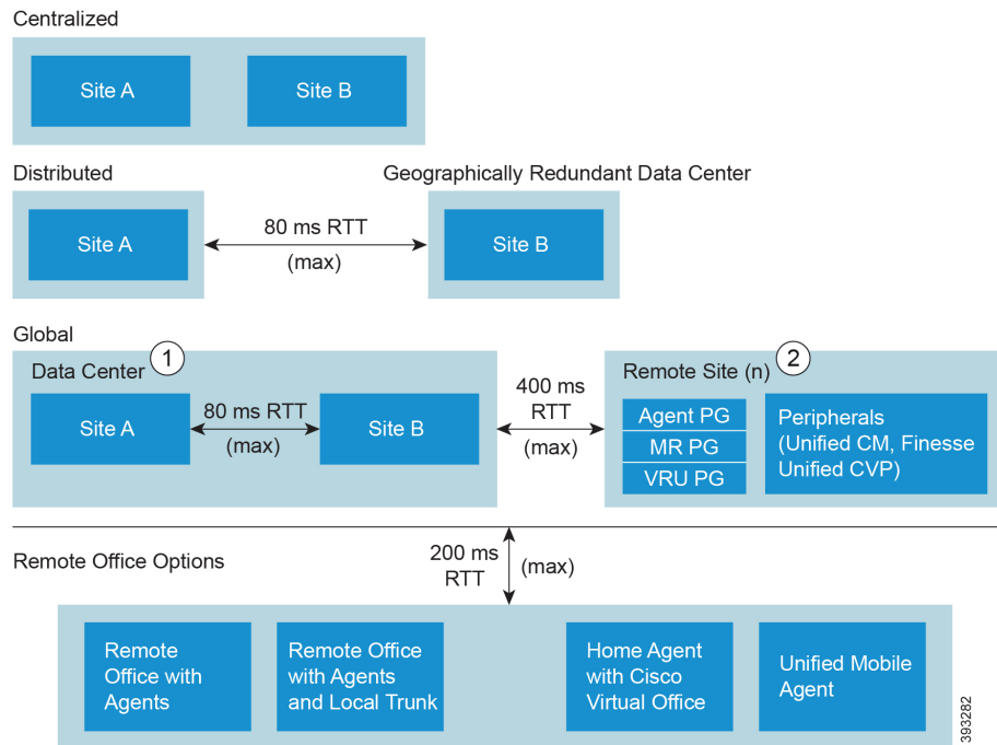
Figure 38: Topologies
