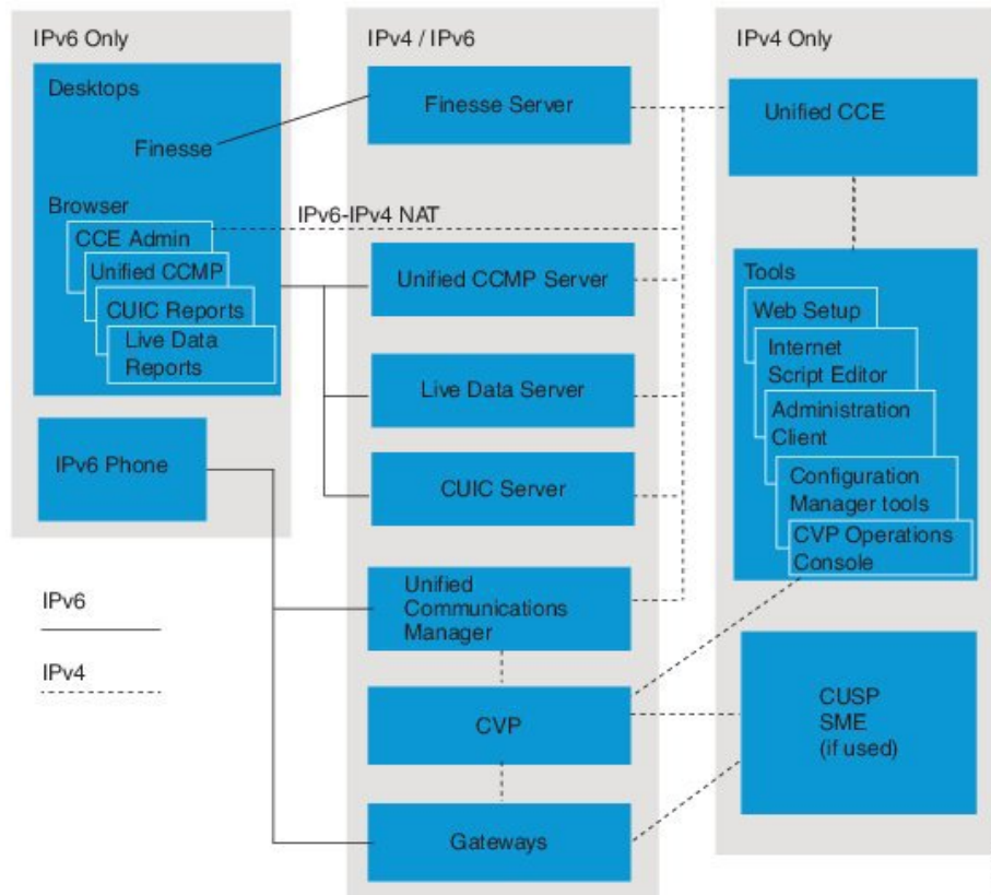
Figure 2: Unified CCE Deployment with Only IPv6 Agents
