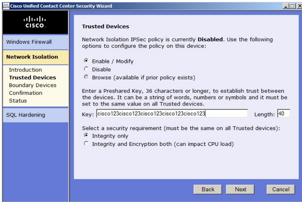
Figure 1: Trusted Devices Configuration Panel
