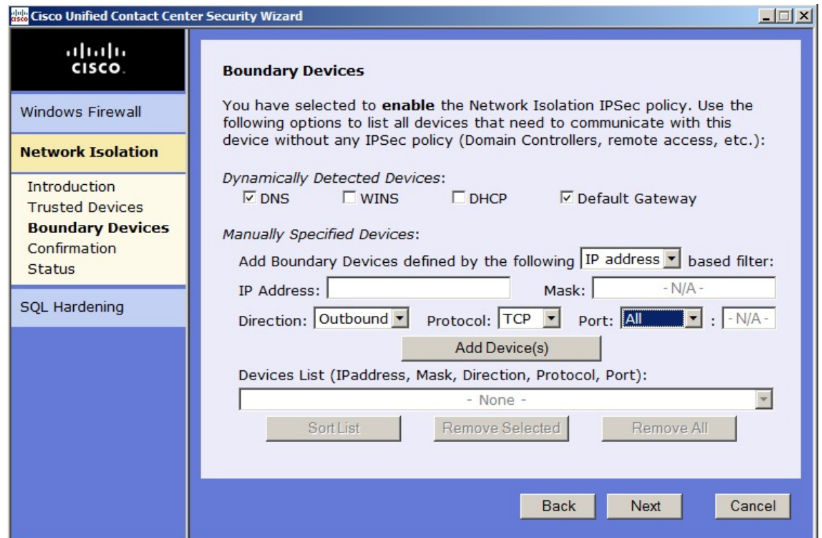
Figure 2: Boundary Device Configuration Panel
