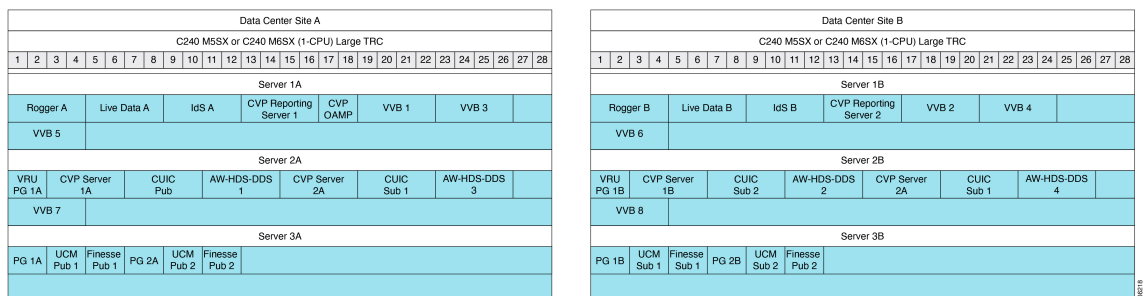
Figure 7: Small Contact Center Shared Peripheral Option
