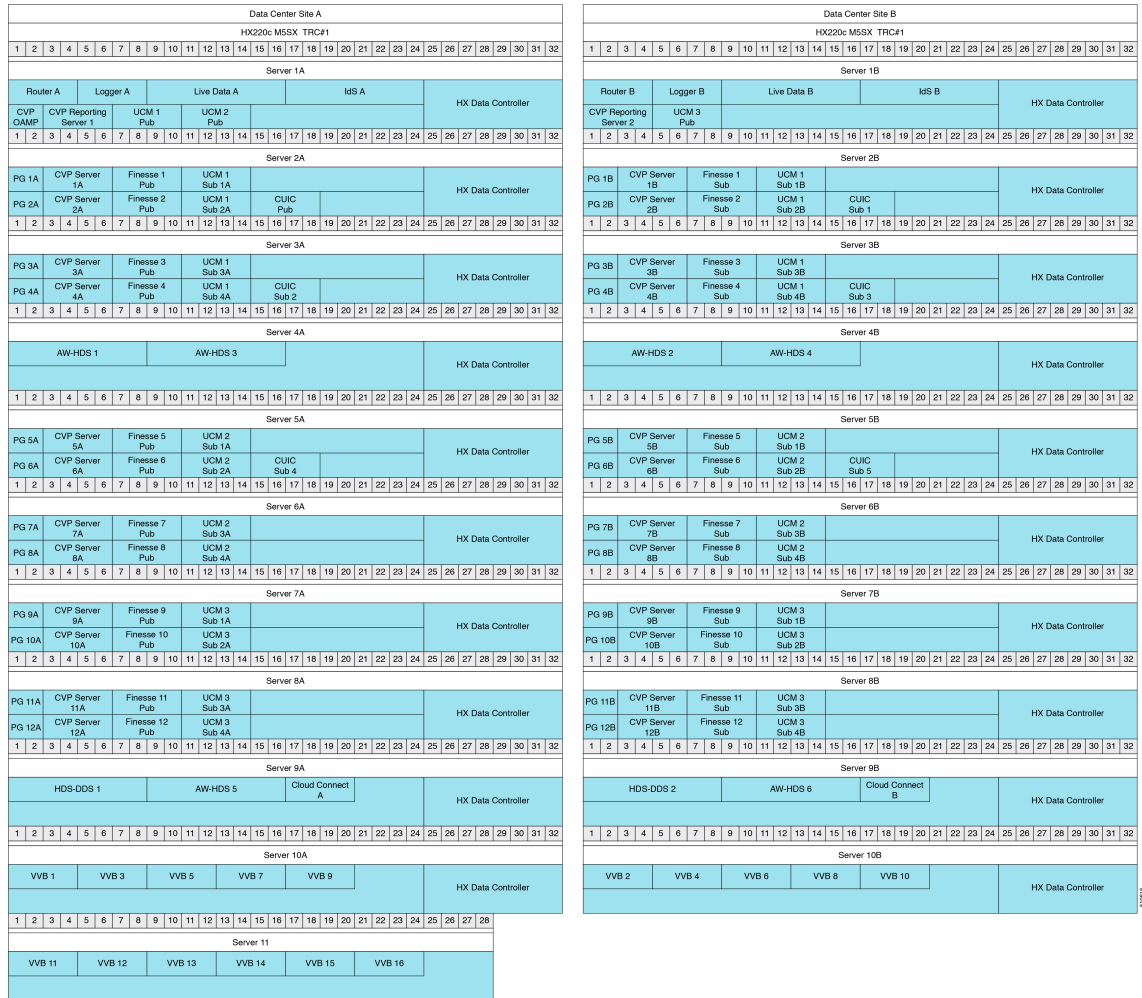
Figure 16: 24000 Agent Reference Design Model
