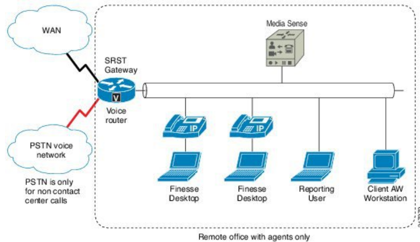
Figure 44: Remote Office with Agents—Physical View
