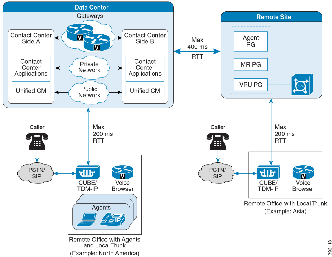
Figure 41: Remote CVP Deployment Topology
