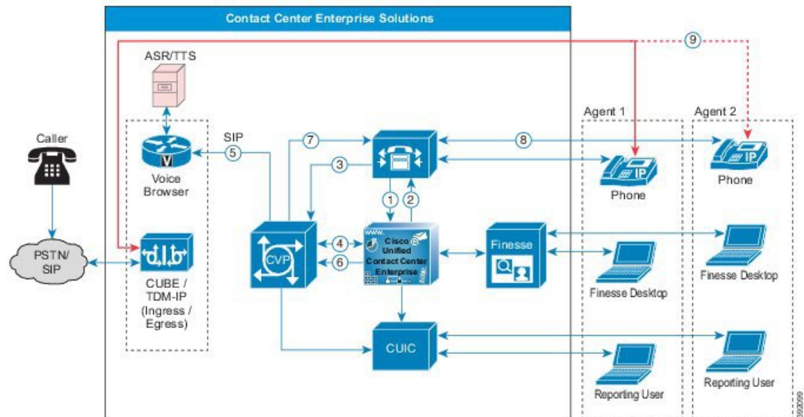
Figure 35: Blind Transfer Call Flow with VRU and Queue to a Second Agent
