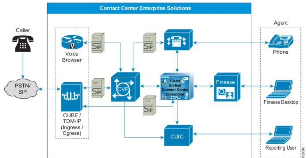
Figure 24: CUSP in a Contact Center Enterprise Solution
