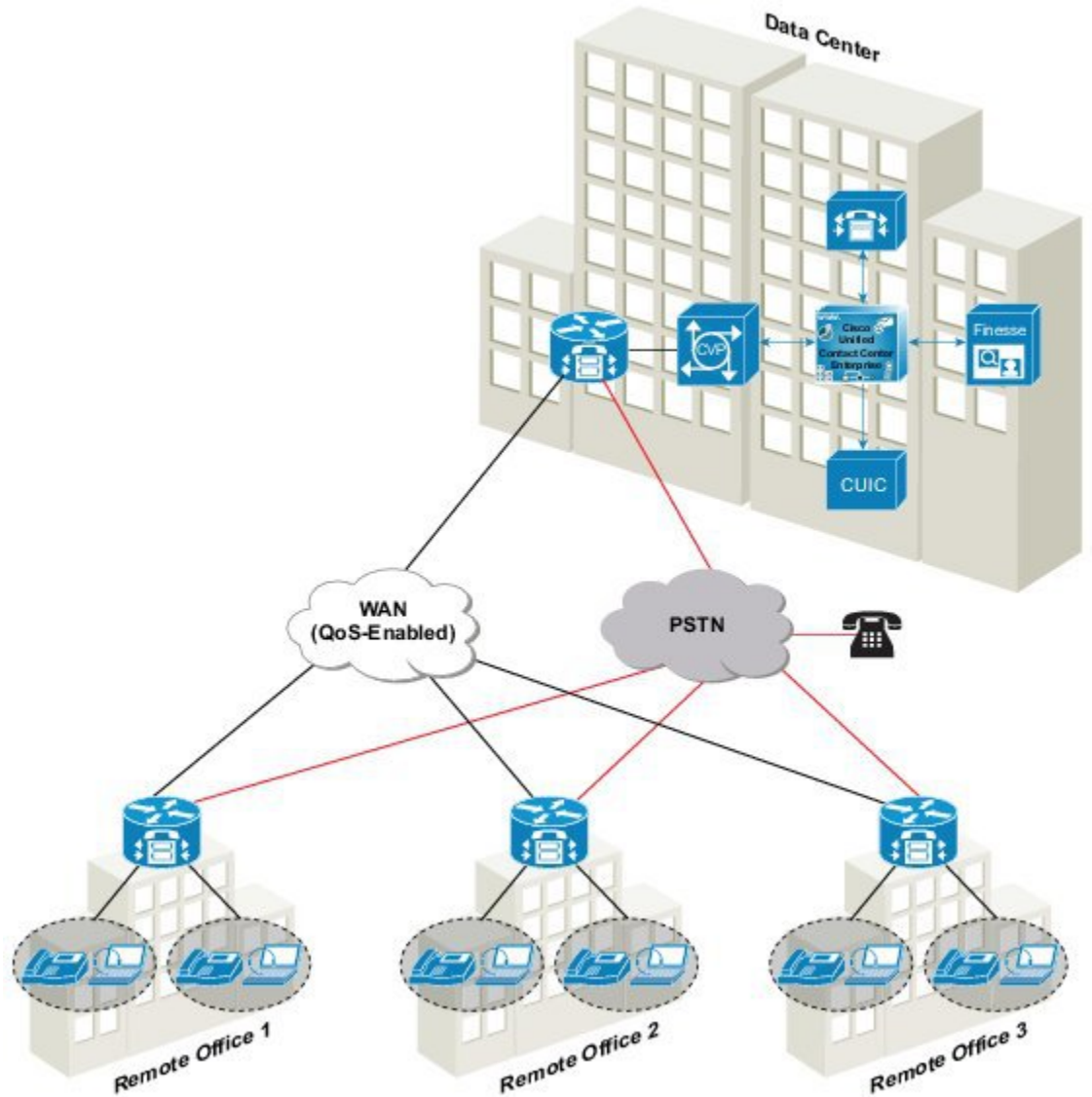
Figure 45: Remote Offices with Agents and Local Trunks
