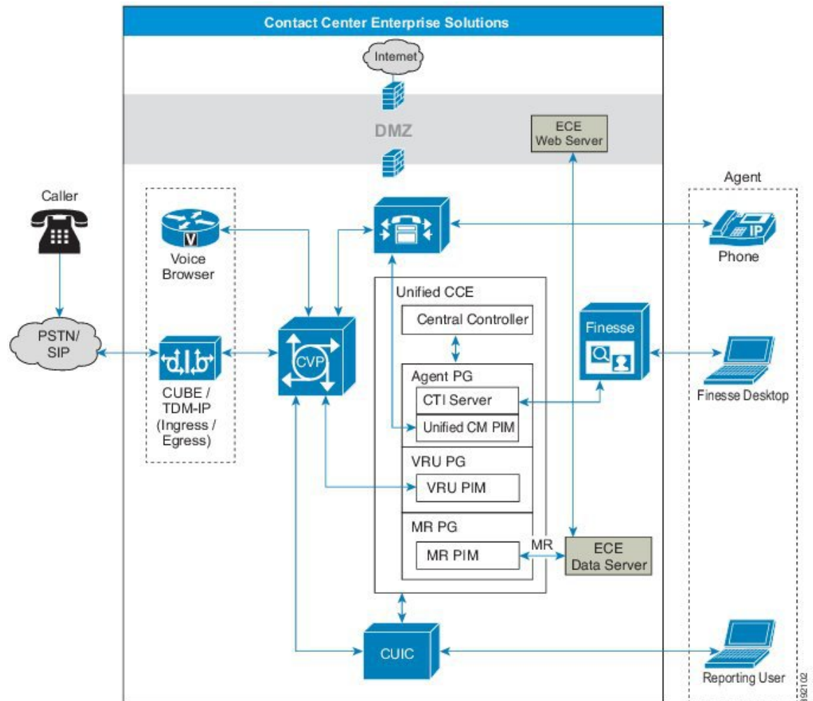
Figure 25: ECE in Contact Center Enterprise Solutions
