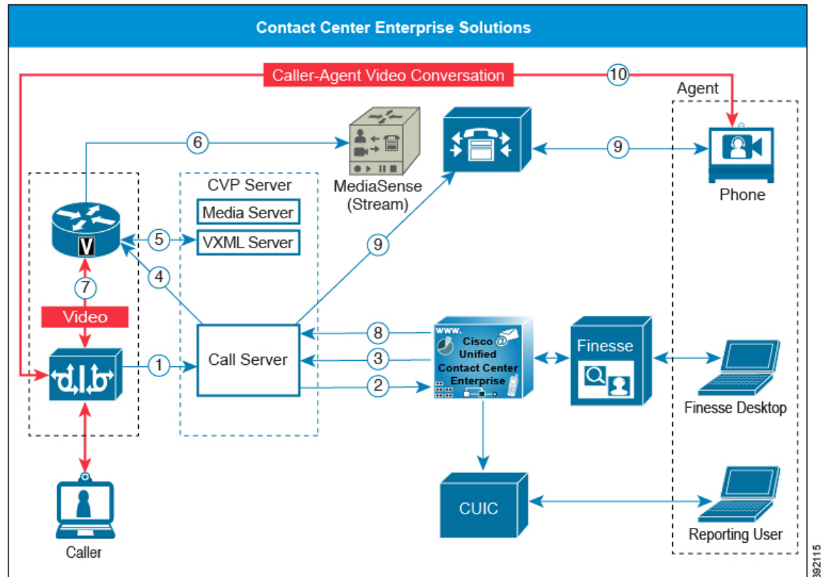
Figure 34: Video Call Flow
