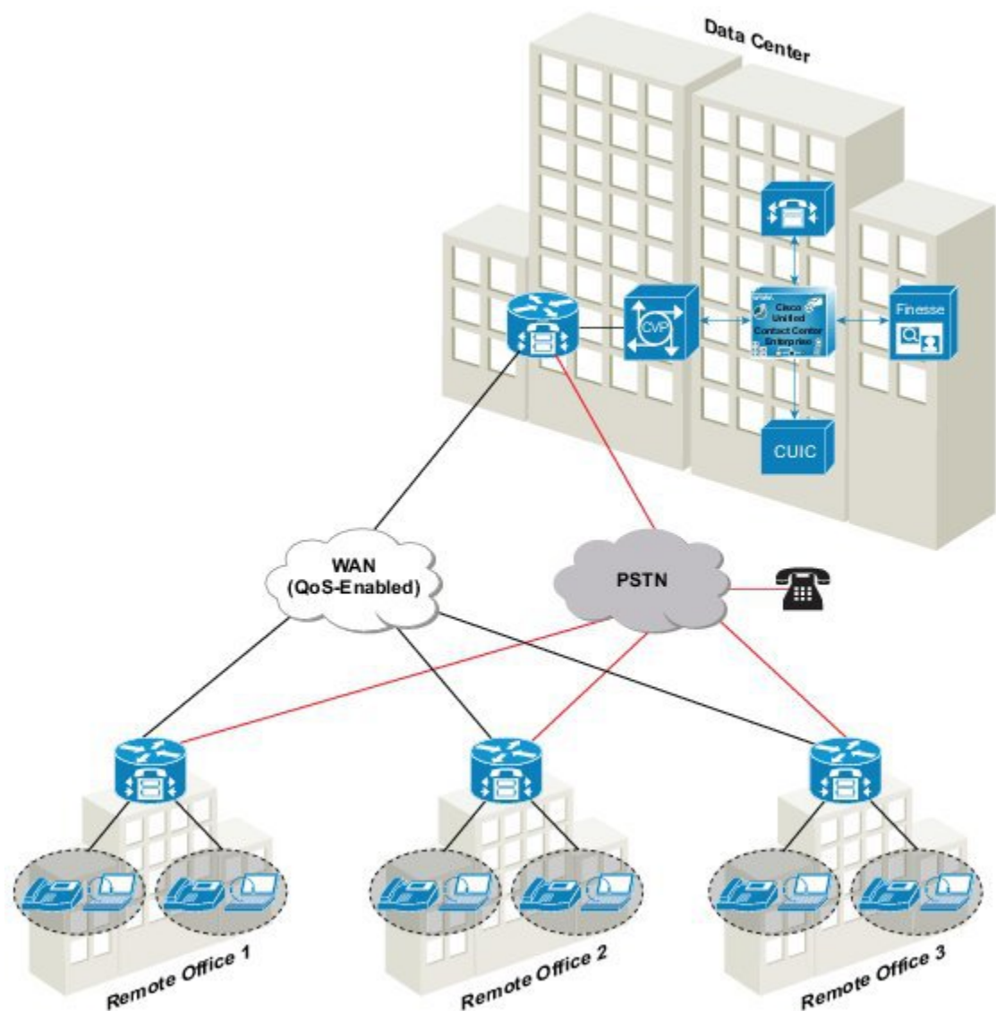
Figure 47: Typical Branch Office Deployment.
