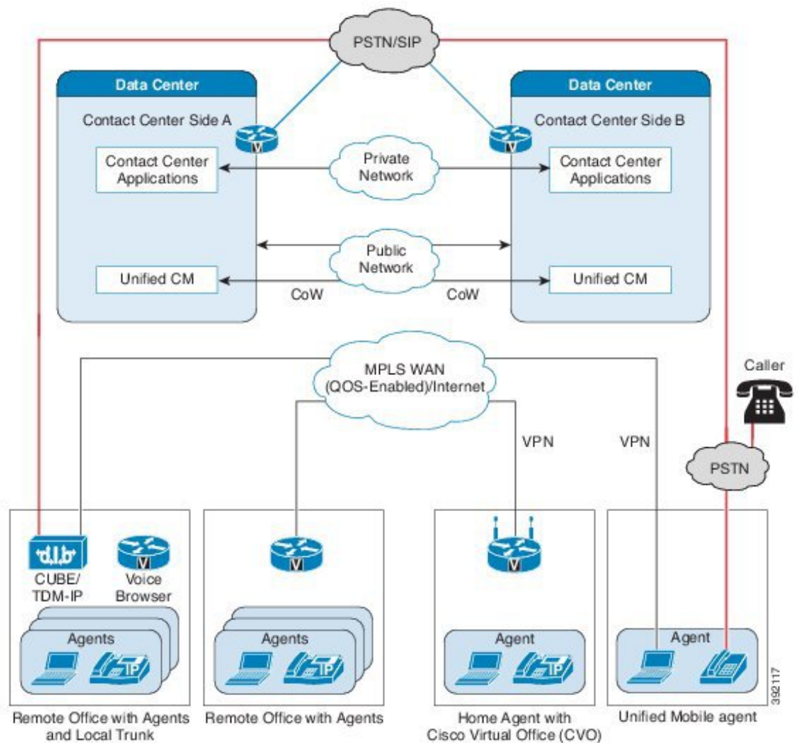
Figure 40: Geographically Redundant Sites with Clustering over WAN
