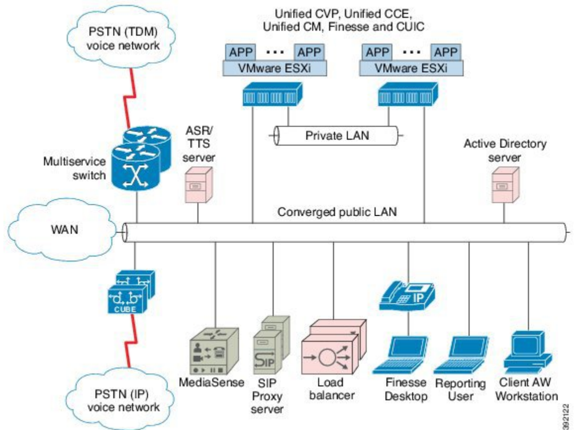
Figure 39: Local Agent—Physical View
