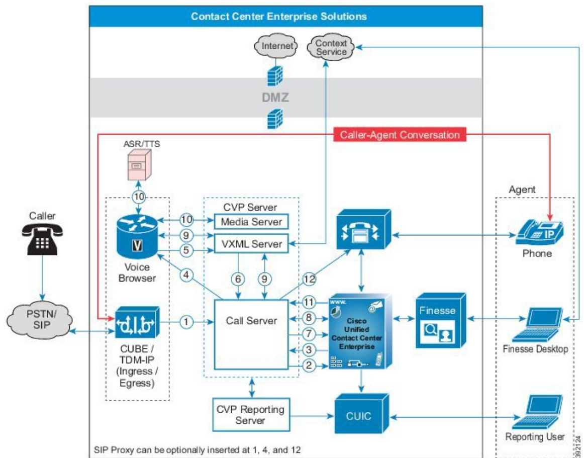
Figure 33: Detailed Call Flow for New Incoming Call
