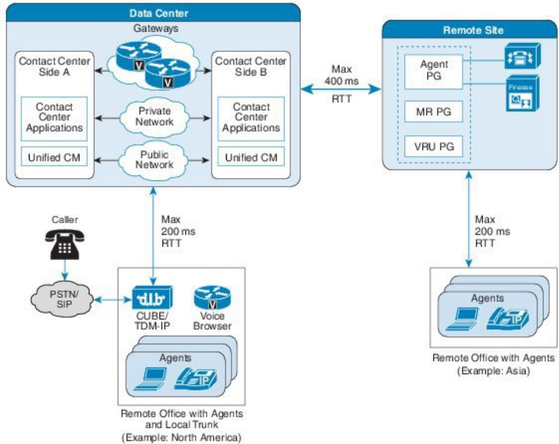
Figure 42: Remote Unified Communications Manager Clusters Topology
