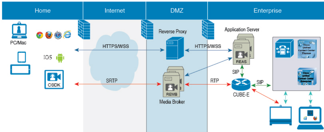
Figure 22: Remote Expert Mobile Deployment
