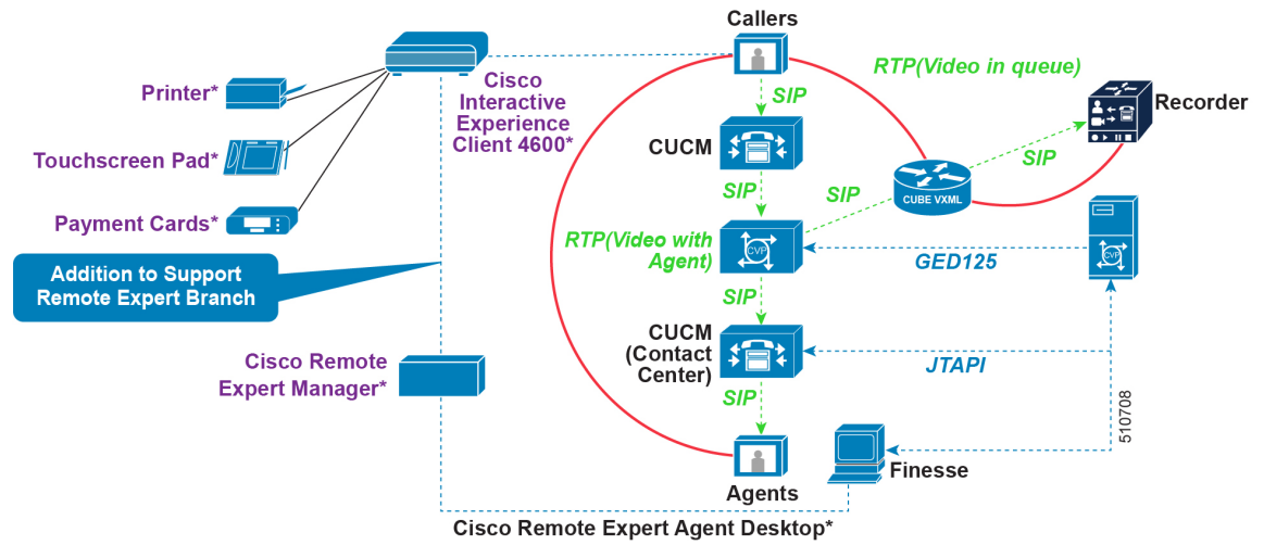
Figure 20: Remote Expert Branch—Immersive/Kiosk Mode
