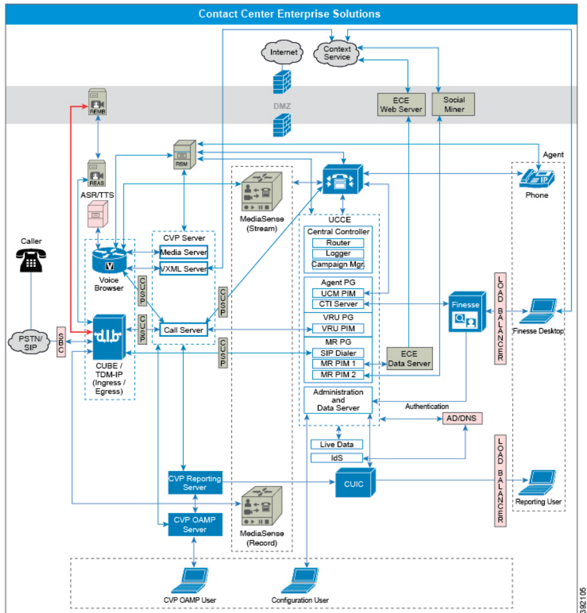
Figure 30: Logical Component Connectivity
