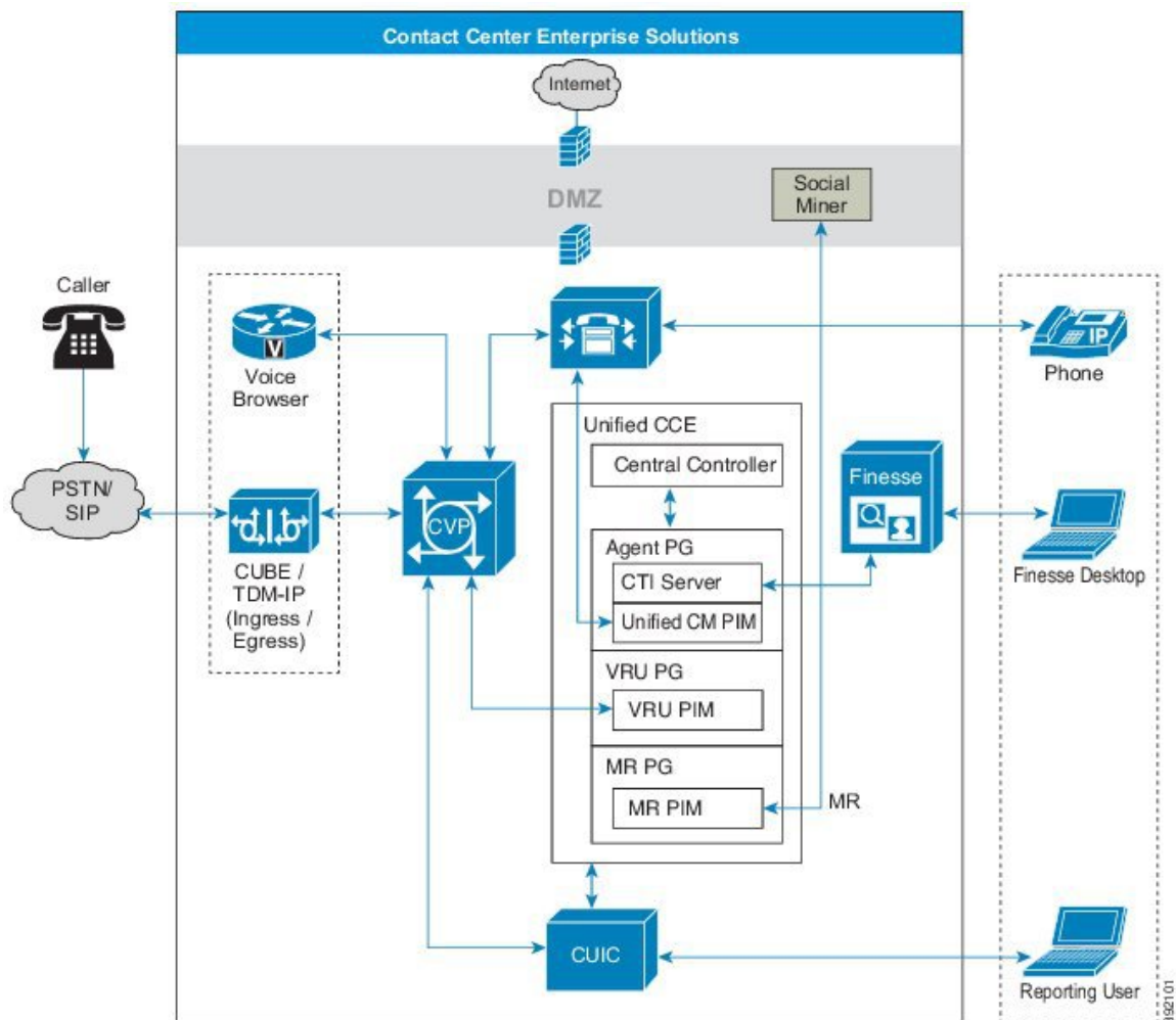
Figure 23: Social Miner in Contact Center Enterprise Solutions
