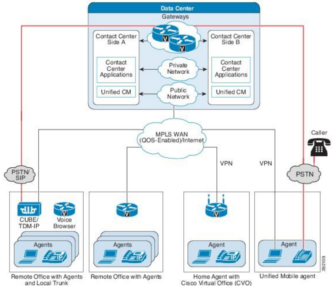
Figure 37: Contact Center Enterprise Solution Topology and Remote Office Options
