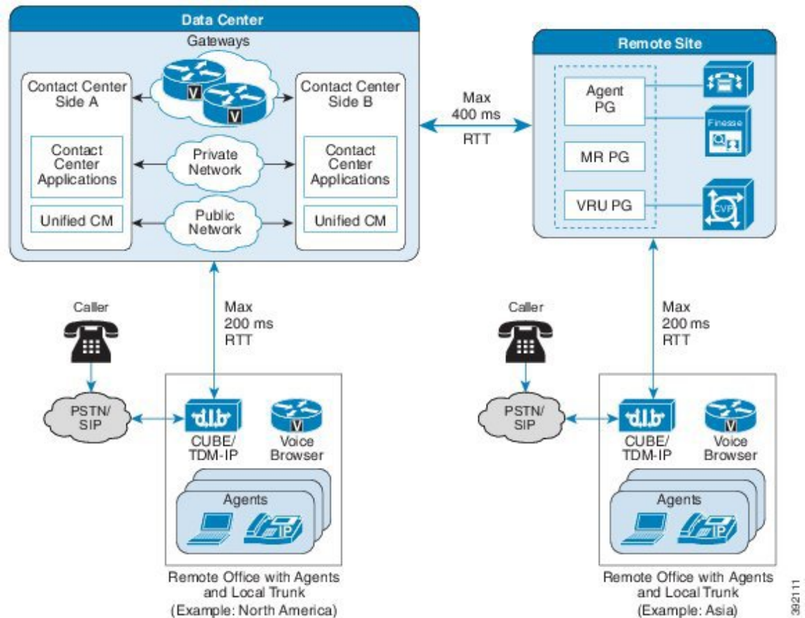
Figure 43: Global Deployment Topology
