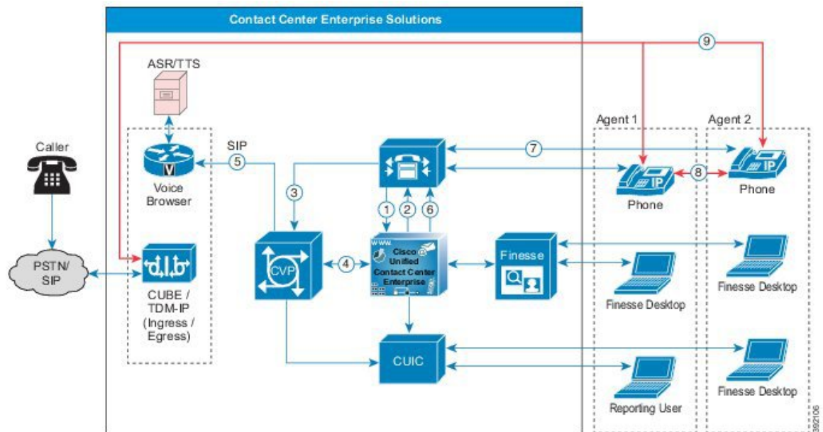
Figure 36: Consult Call Flow with VRU and Queue to a Second Agent
