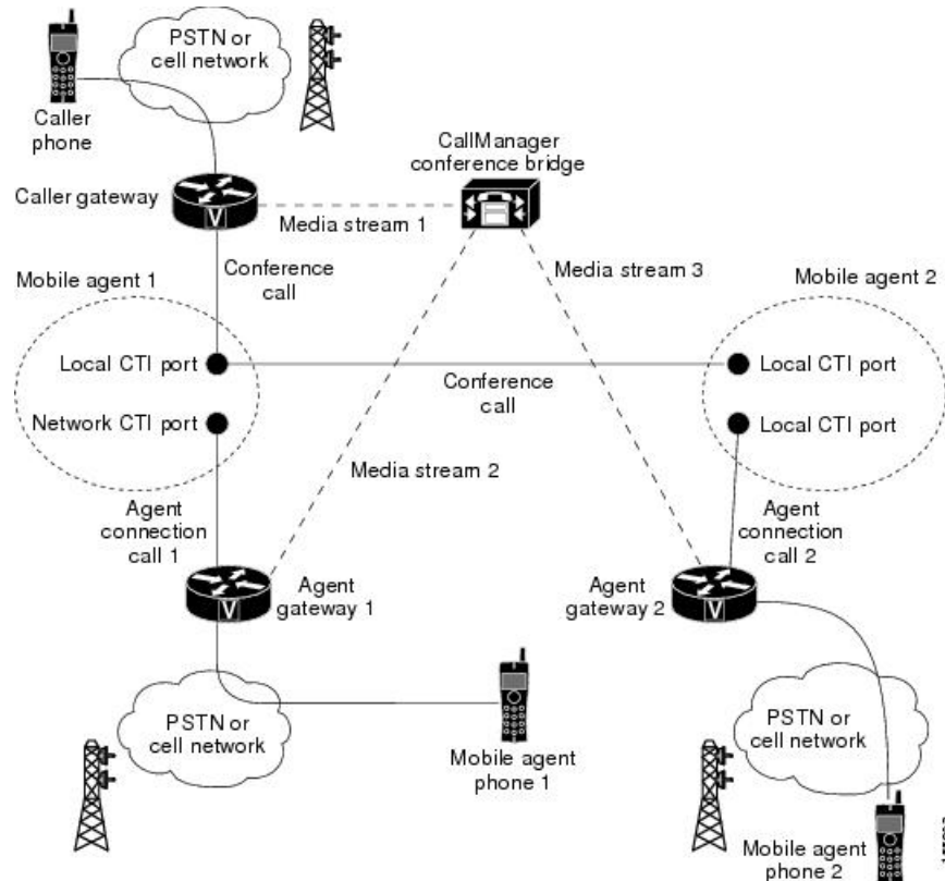
Figure 6: Mobile Agent Remote Conference Call Flow
