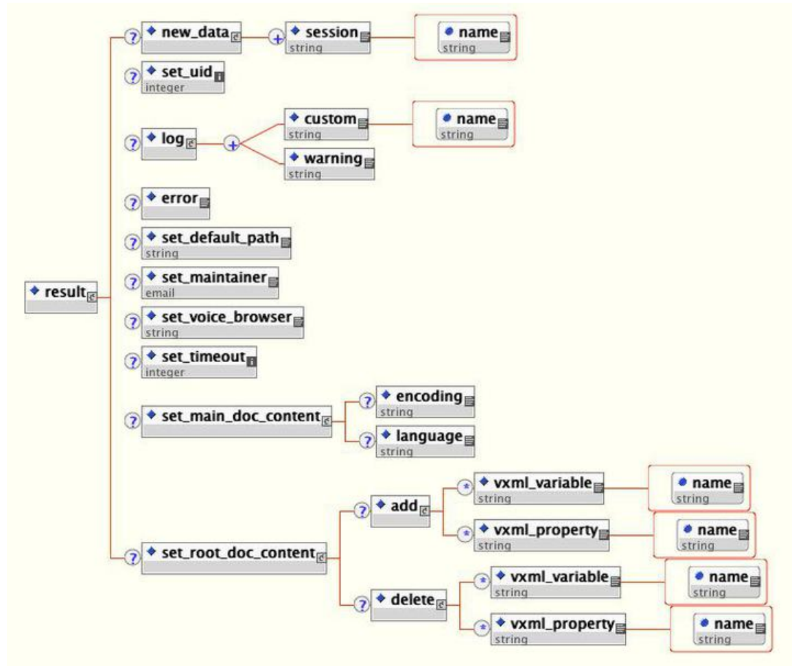
Figure 1: DTD Diagram of XML Document to Be Sent in Response
