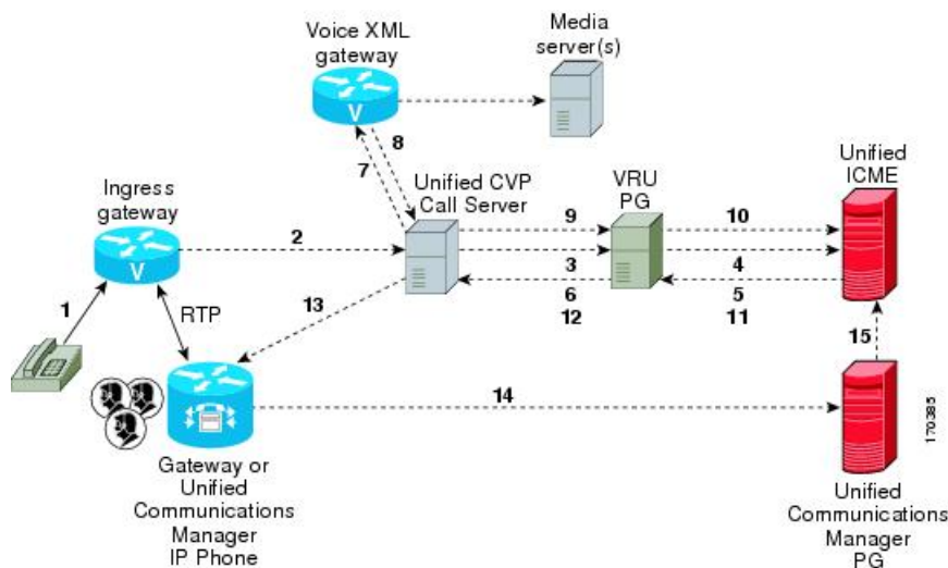
Figure 2: Comprehensive Call Flow Model for ICME Using SIP Without a Proxy Server
