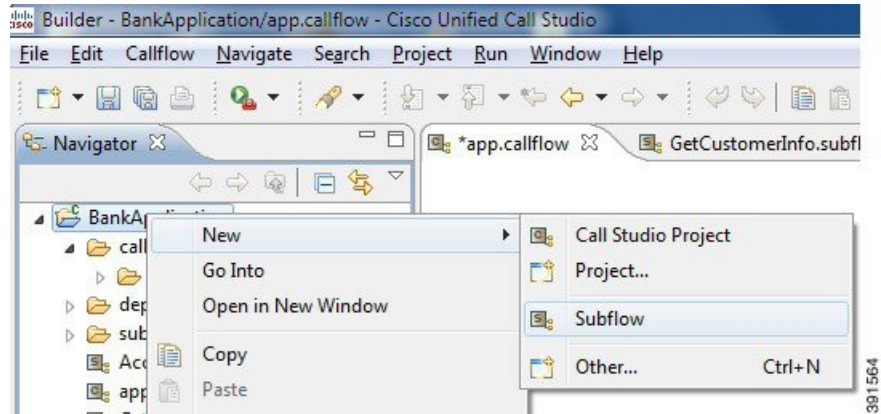
Figure 11: Create Subflow
