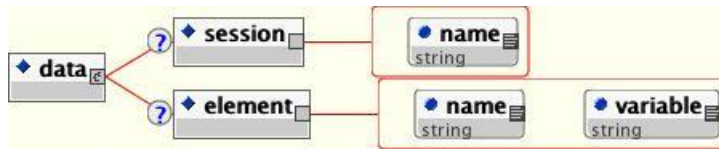
Figure 18: data Tag
