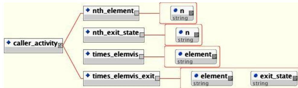
Figure 21: caller_activity Tag
