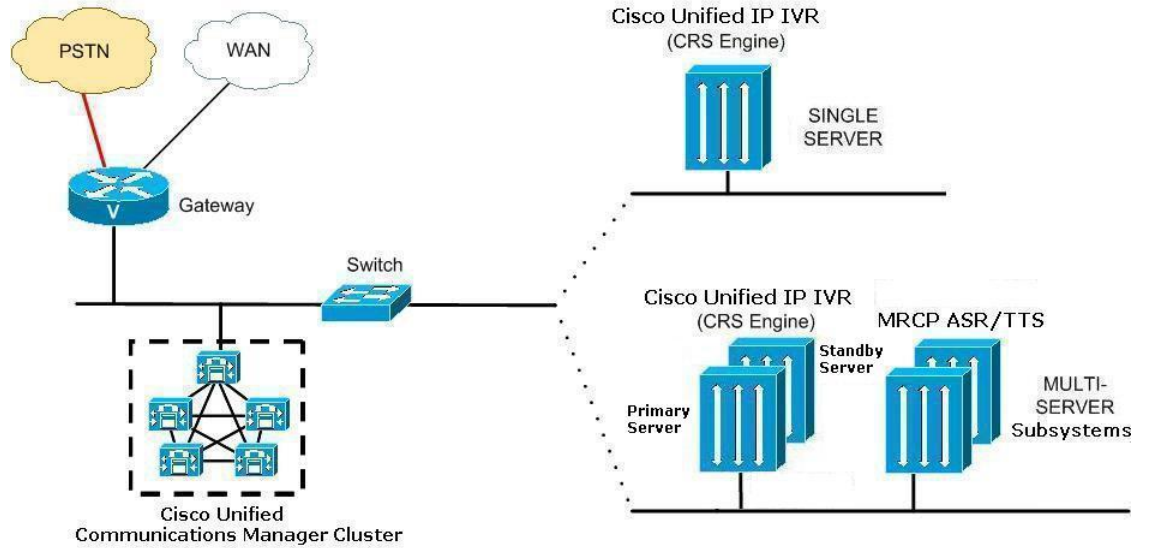
Figure 2: Standalone Deployment Model for Unified IP IVR
