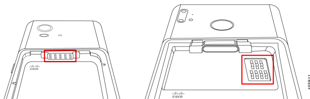
Figure 6: Battery contact location on the Cisco Wireless Phone 840 and Cisco Wireless Phone 860
