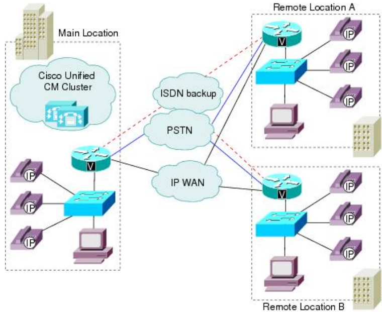
Figure 1: Call admission control that uses locations in a centralized system
