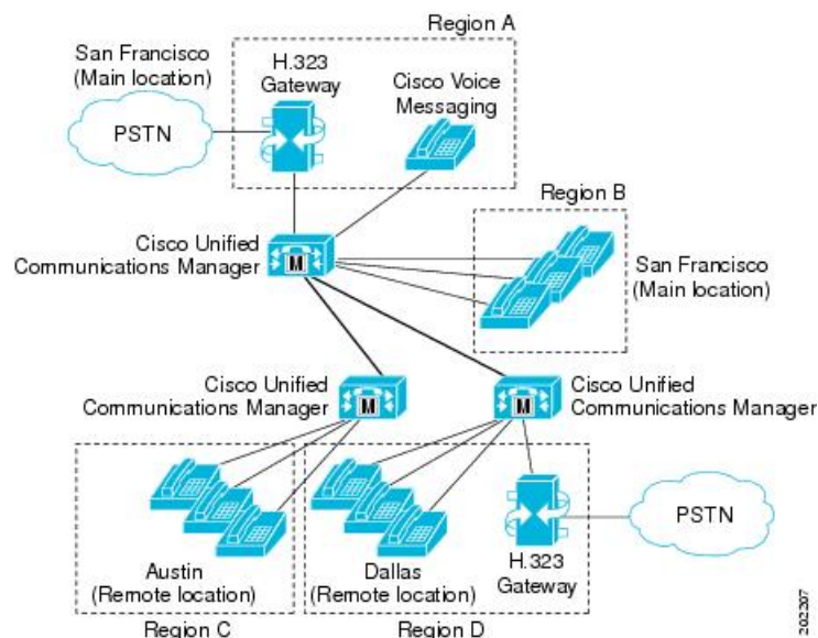
Figure 2: Interaction among locations and regions
