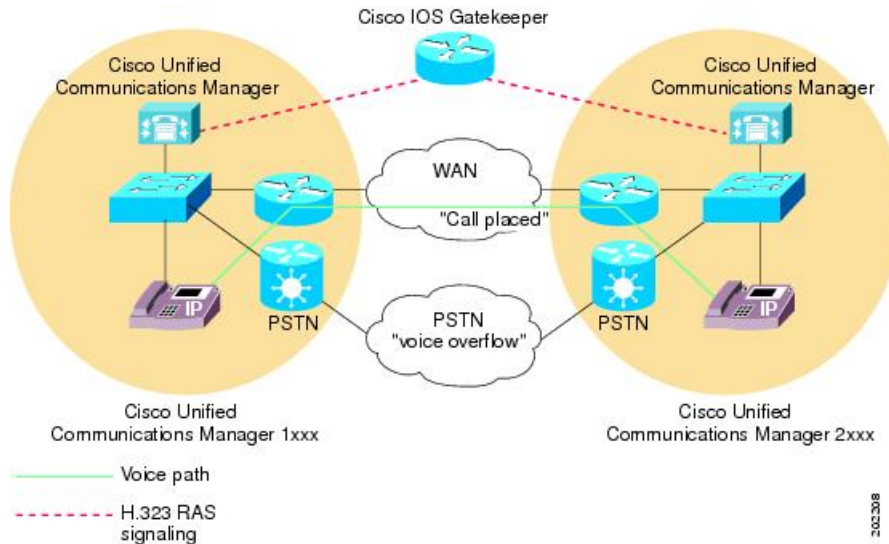
Figure 3: Call admission control by using a gatekeeper in a distributed system
