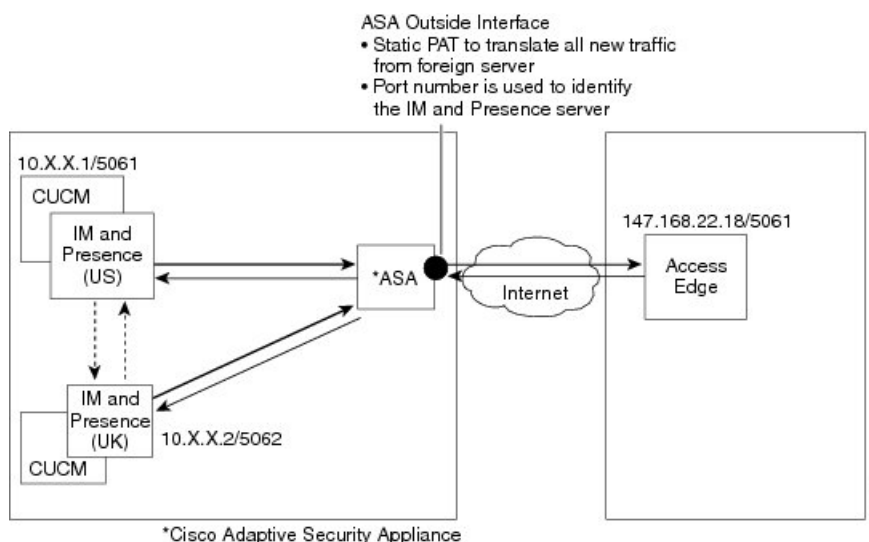
Figure 3: Static PAT for Messages Originating From an External Domain
