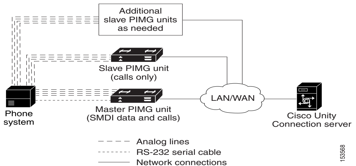
Figure 21-1 Connections for a Serial MD-110 Integration Using Analog PIMG Units
