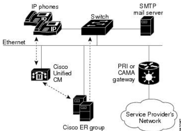
Figure 4: How Cisco Emergency Responder Fits Into Your Network
