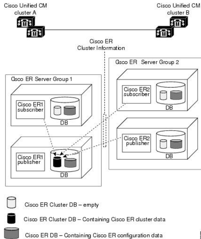
Figure 10: Understanding the Relationship Between Cisco Emergency Responder Groups and CiscoEmergency Responder Clusters
