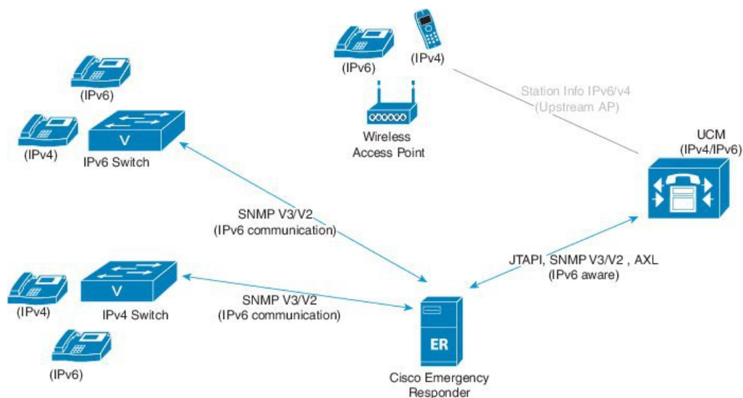
Figure 1: IPv6 Endpoints
