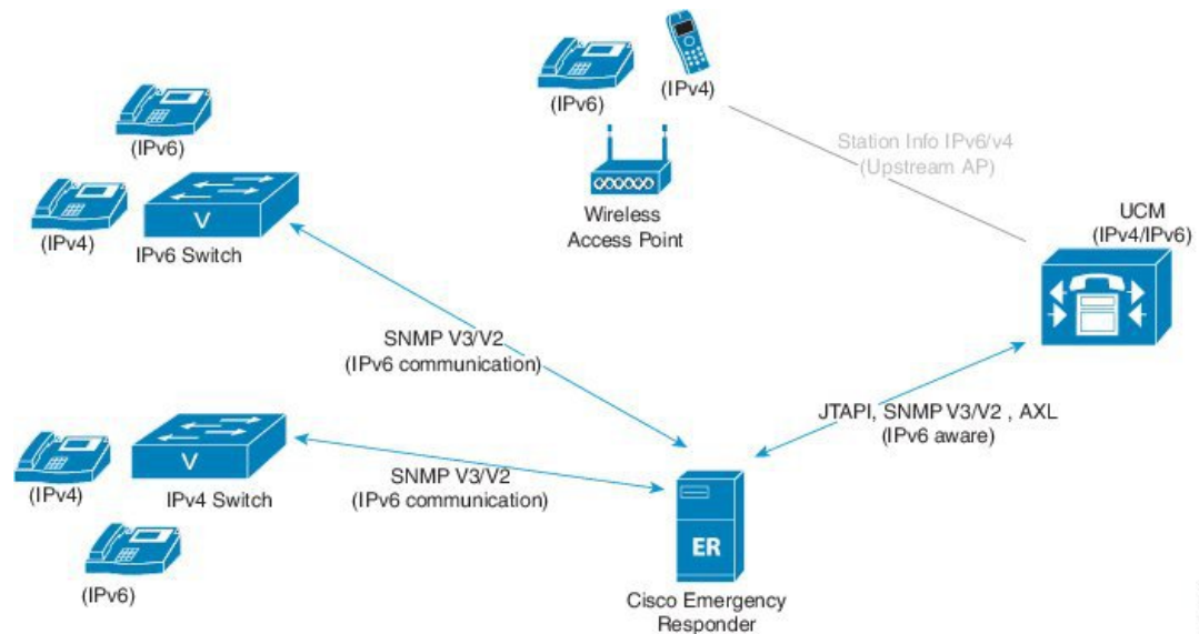
Figure 1: IPv6 Endpoints
