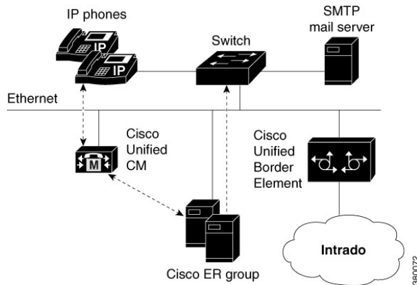
Figure 7: Cisco Emergency Responder and Intrado
