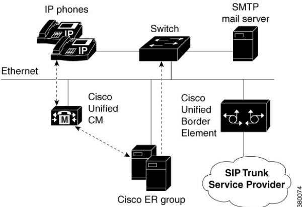
Figure 3: Cisco Emergency Responder and a SIP Trunk Service Provider
