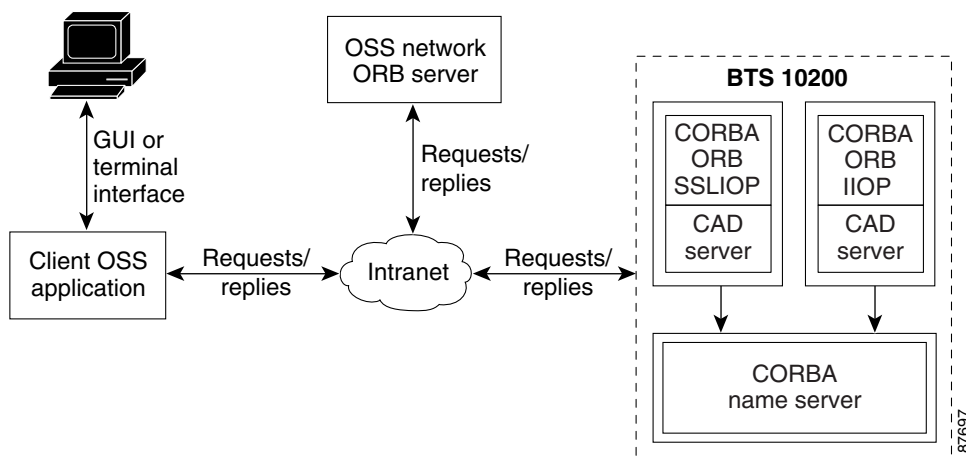
Figure 1-1 CORBA Architecture
