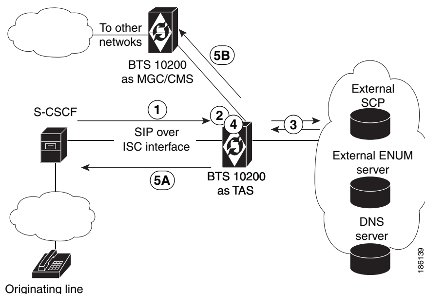
Figure 1-16 Example of Origination + Routing Request—Call with OCB Screening
