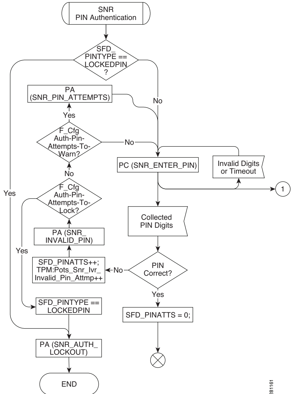
Figure 5-3 PIN Authentication
