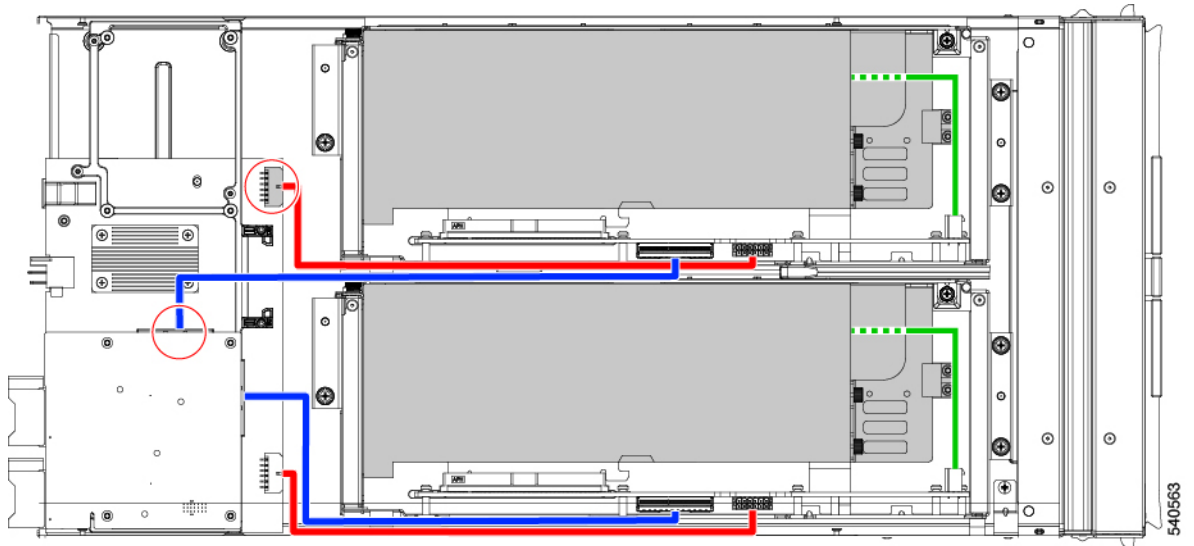
Figure 3: PCB Cable Connectors, FHFL GPU
