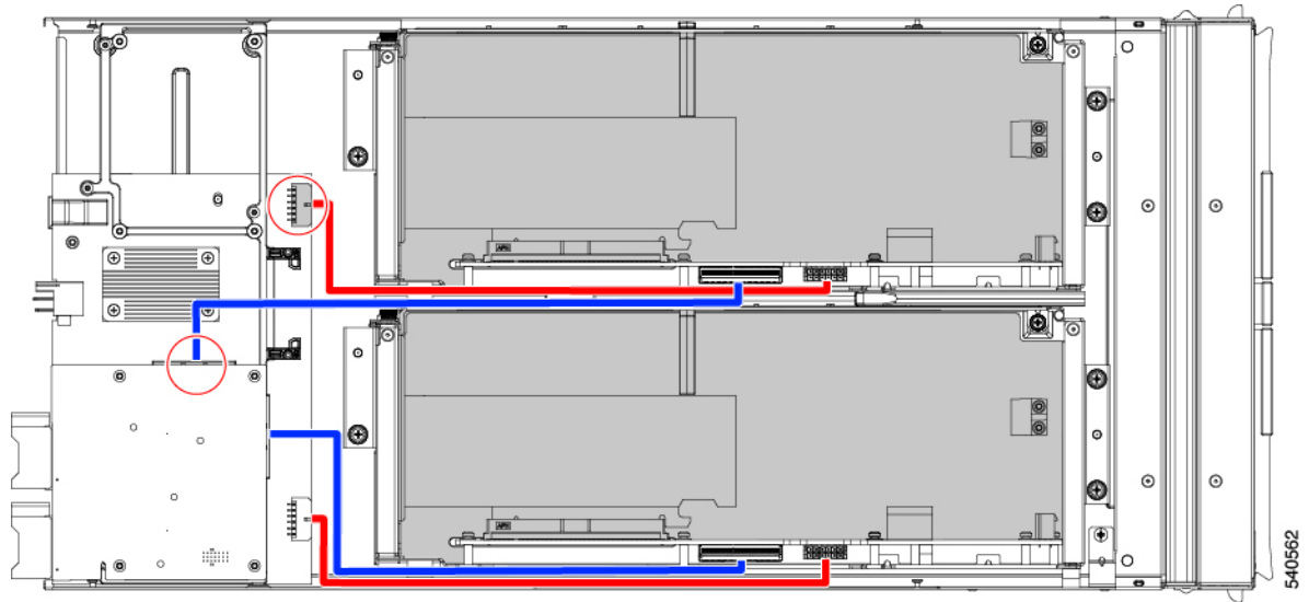
Figure 4: PCB Cable Connectors, HHHL GPU
