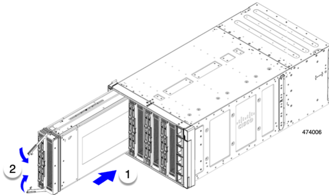
Figure 5: Installing a Cisco UCS X410c M7 Compute Node
