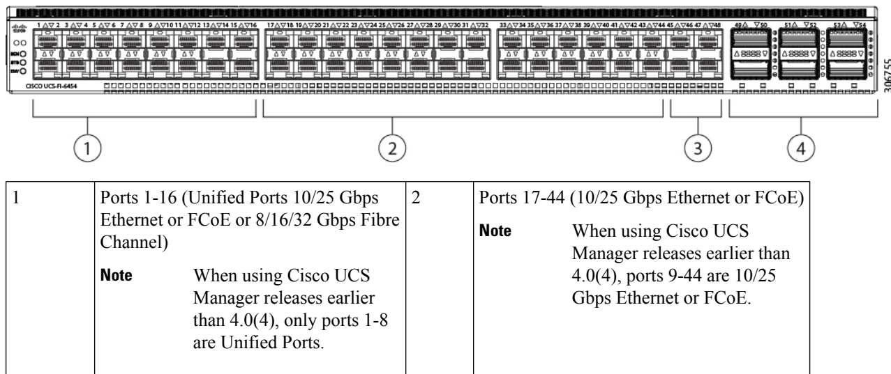
Figure 7: Cisco UCS 6454 Fabric Interconnect Rear View
