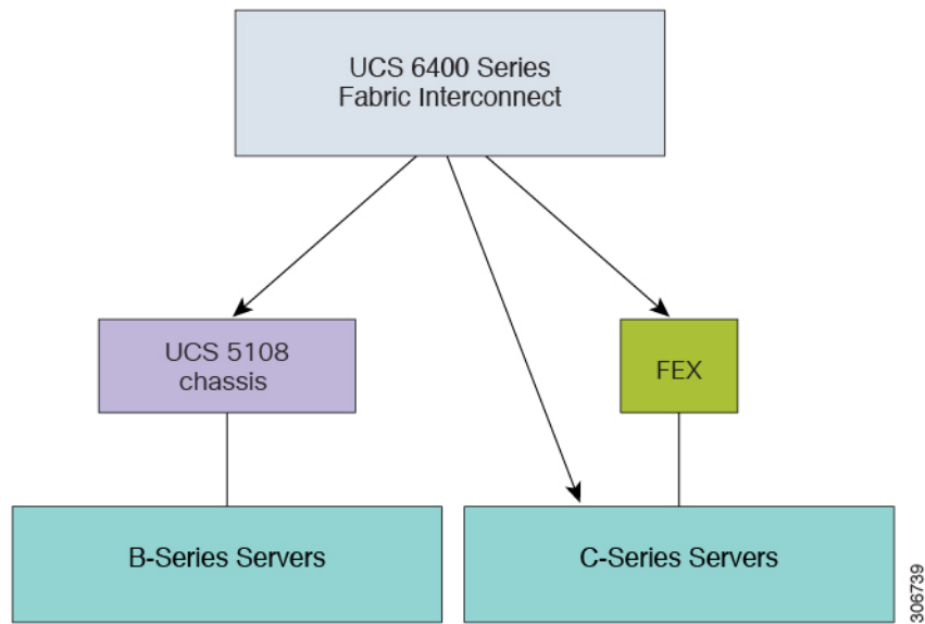
Figure 2: Cisco UCS 6400 Series Fabric Interconnect with Cisco UCS B-Series and C-Series servers
