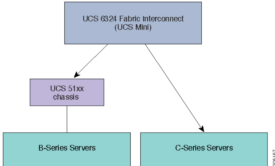
Figure 5: Cisco UCS 6324 Fabric Interconnect with Cisco UCS B-Series Servers and C-Series servers
