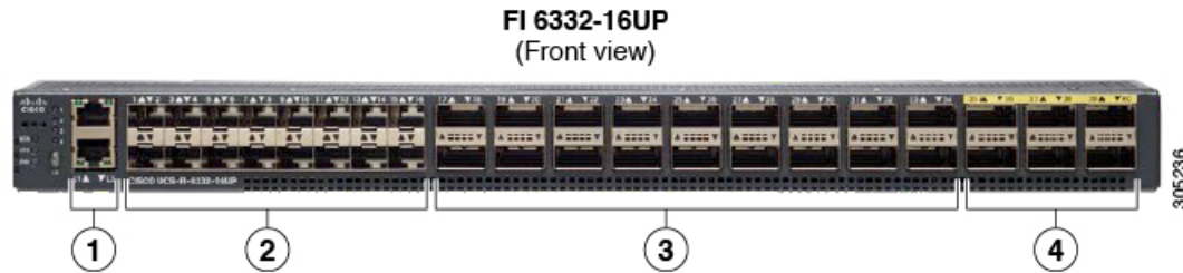
Figure 3: Cisco UCS 6332-16UP Series Fabric Interconnects Front View
