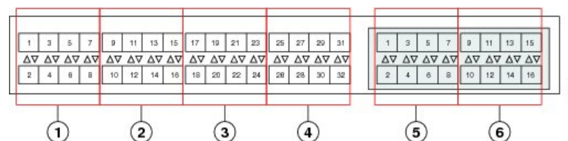
Figure 5: Port Groups for Fabric Port Channels
