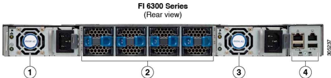
Figure 4: Cisco UCS 6300 Series Fabric Interconnects Rear View
