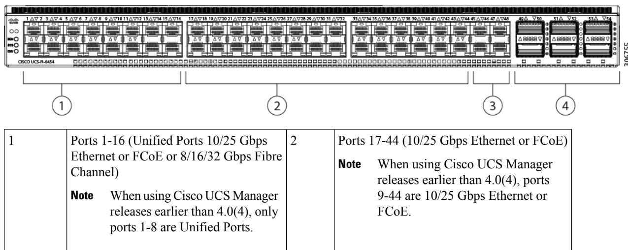
Figure 7: Cisco UCS 6454 Fabric Interconnect Rear View
