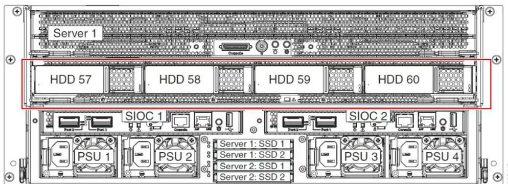
Figure 4: Cisco UCS 3260 with the HDD expansion tray (Rear View)
