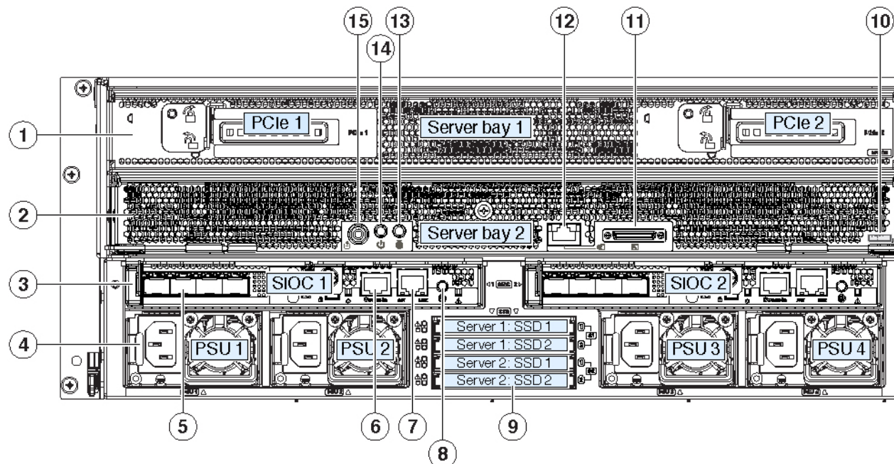
Figure 2: Figure 1-2 Rear Panel Features (S3260 M5 Server Node With I/O Expander and Version 03 SIOCs Shown)
