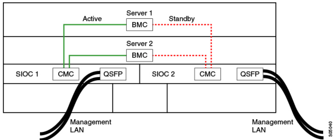
Figure 6: Figure 1-6 Management Architecture
