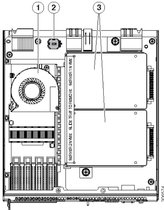
Figure 5: Figure 1-5 Replaceable Components Inside the Version 03 SIOC (UCS-S3260-PCISIOC)
