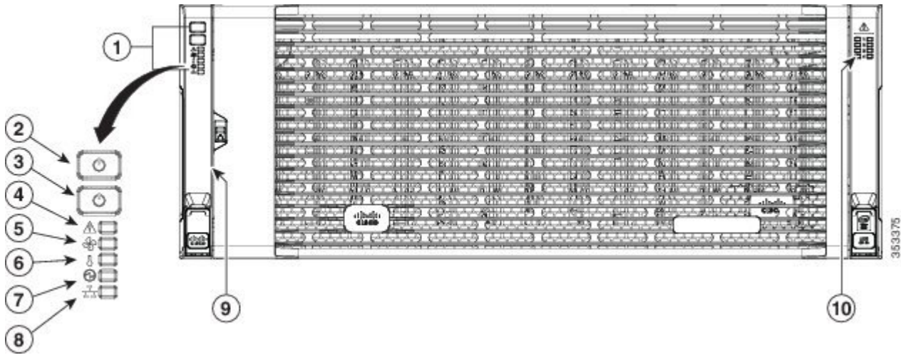
Figure 1: Figure 1-1 Front Panel Features
