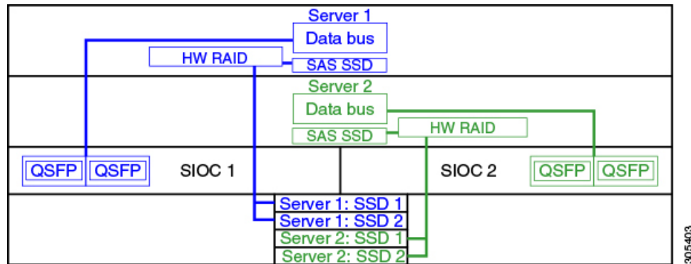
Figure 8: Figure 1-8 Data Architecture in a Dual-Server System
