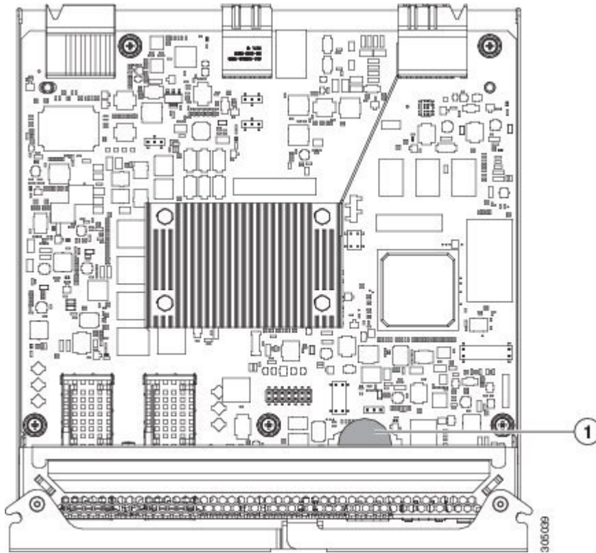
Figure 4: Figure 1-4 Replaceable Components Inside the Version 02 SIOC (UCSC-S3260-SIOC)
