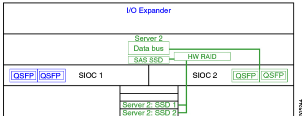
Figure 9: Figure 1-9 Data Architecture in a Single-Server System With I/O Expander
