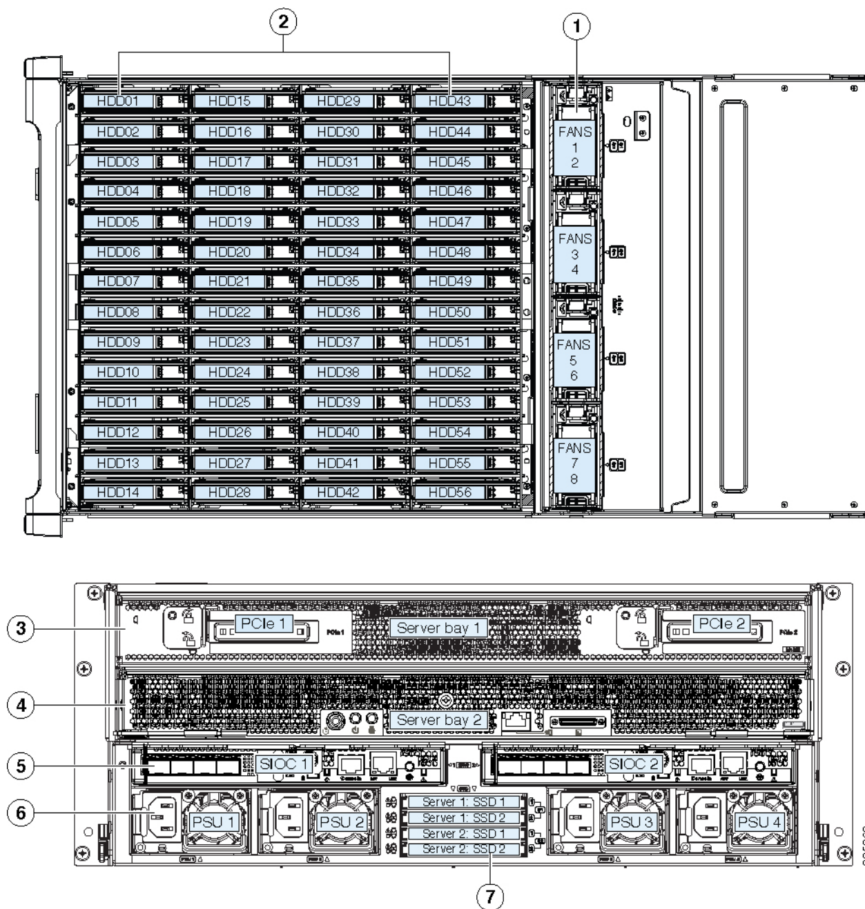
Figure 3: Figure 1-3 Replaceable Components Inside the Main Chassis (Top View and Rear View)
