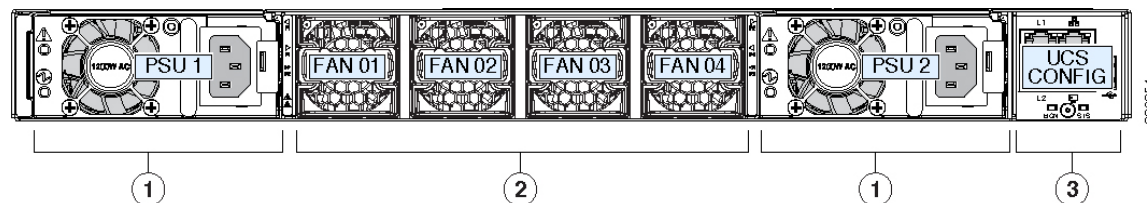
Figure 2: Cisco UCS 6454 Fabric Interconnect Front View
