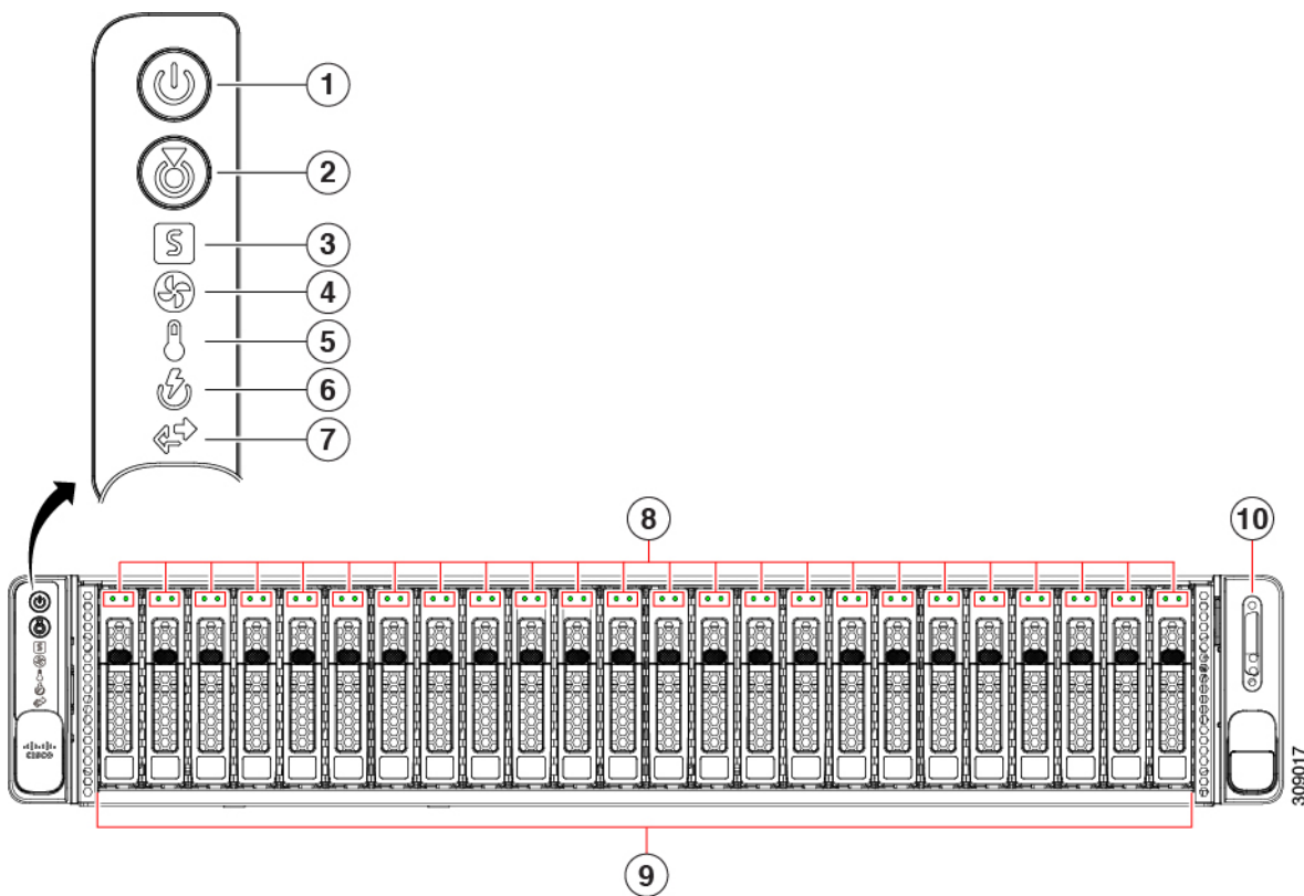
Figure 1: Cisco UCS C240 M6 Server 24 SAS/SATA Front Panel
