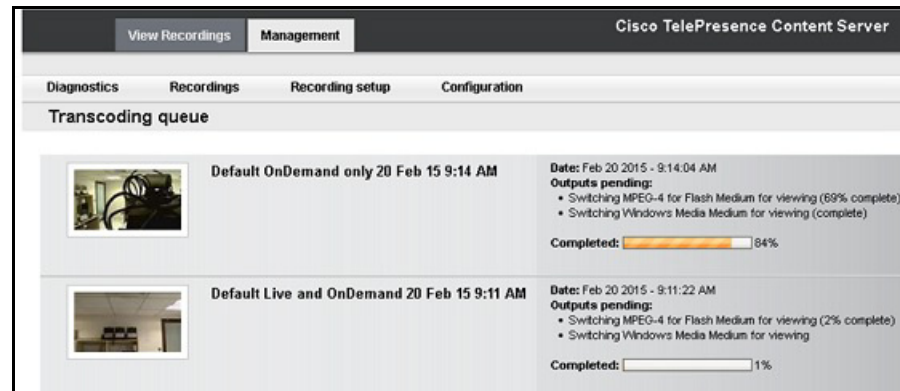
Figure 1-2 Transcoding Queue
