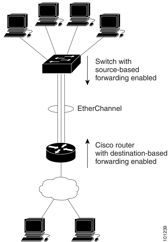
Figure 1-3 Load Distribution and Forwarding Methods
