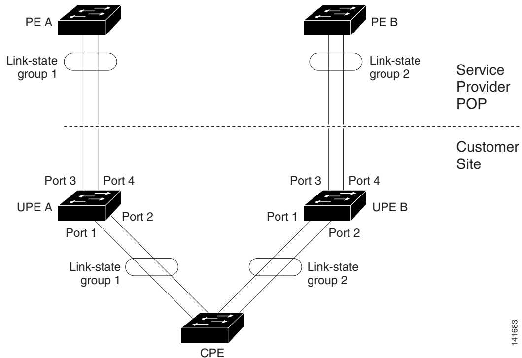
Figure 1-4 Typical Link-State Tracking Configuration
