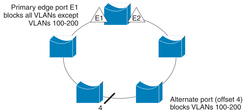
Figure 18-5 Example of VLAN Blocking
